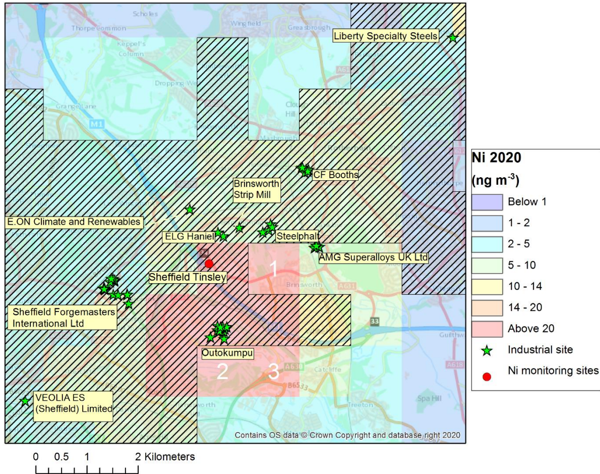
Figure 2. Exceedance situation in Yorkshire and Humberside [Ni_UK0034_2020_1]. The Sheffield Tinsley monitoring station is marked in red. Locations of local industrial sites are also shown. Non-hatched grid squares are assigned to the Yorkshire and Humberside zone UK0034. Note that multiple emissions sources are indicated on the map for some industrial sites (Outokumpu, Sheffield Forgemasters International Ltd, AMG Superalloys UK Ltd, E.L.G. Haniel Metals Limited, Harsco Metals Group Limited (Steelphalt), and CF Booths Limited).
