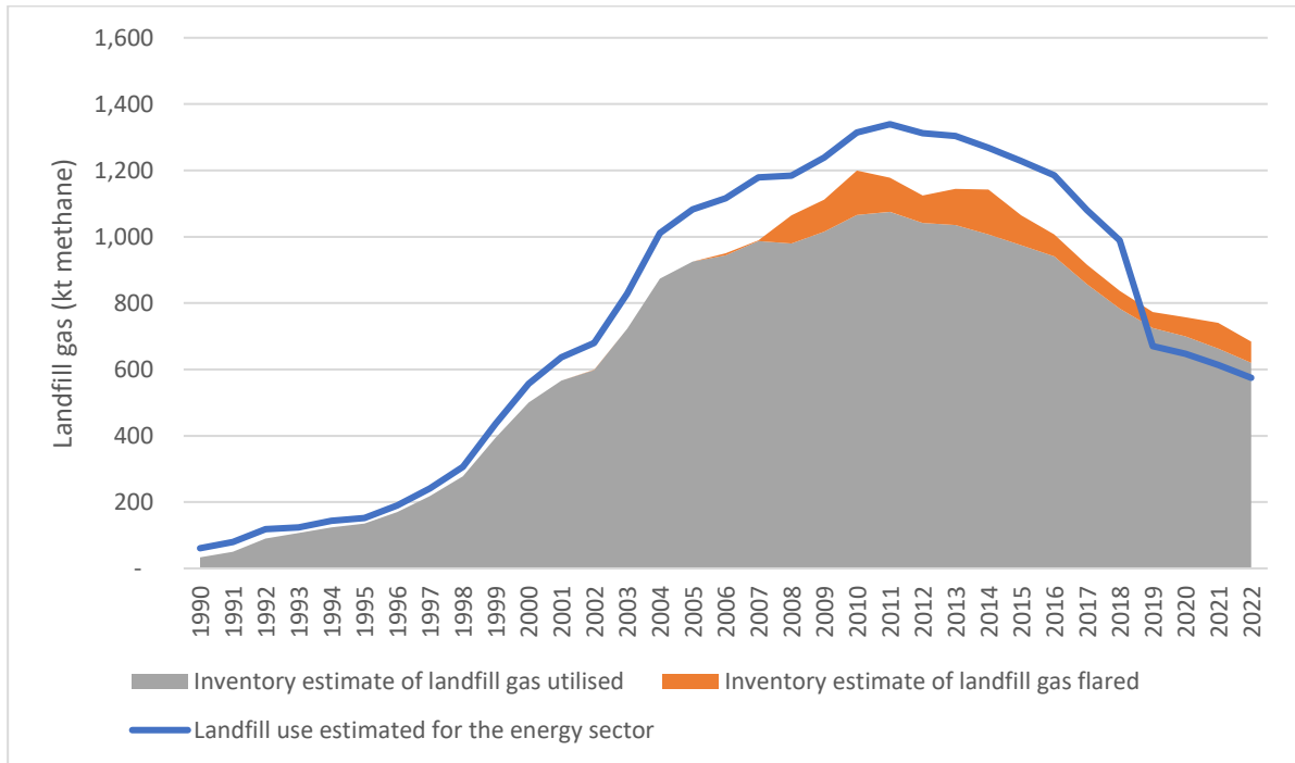
Figure 7.7 Comparison of Estimates of Landfill Gas Utilisation
