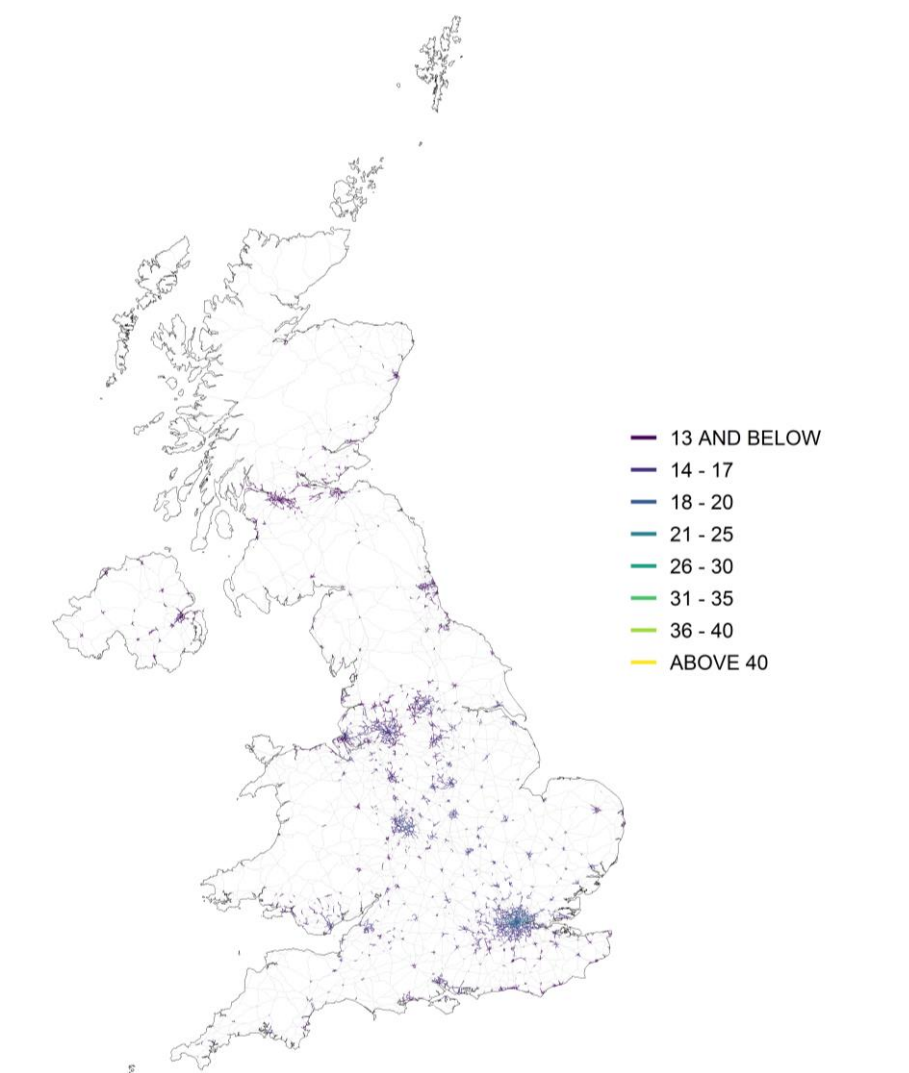
Figure 6.2 - Urban major roads, annual mean roadside PM 10 concentration, 2021 (µg m -3 , gravimetric)
