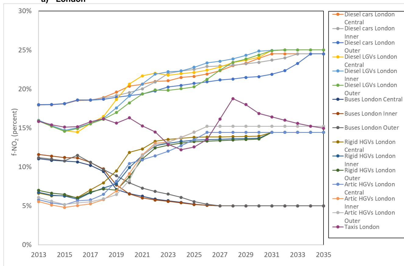
Figure 4.10 - Fleet average f\text{-NO}_2 projections by vehicle type for a) London and b) rest of the UK from NAEI
