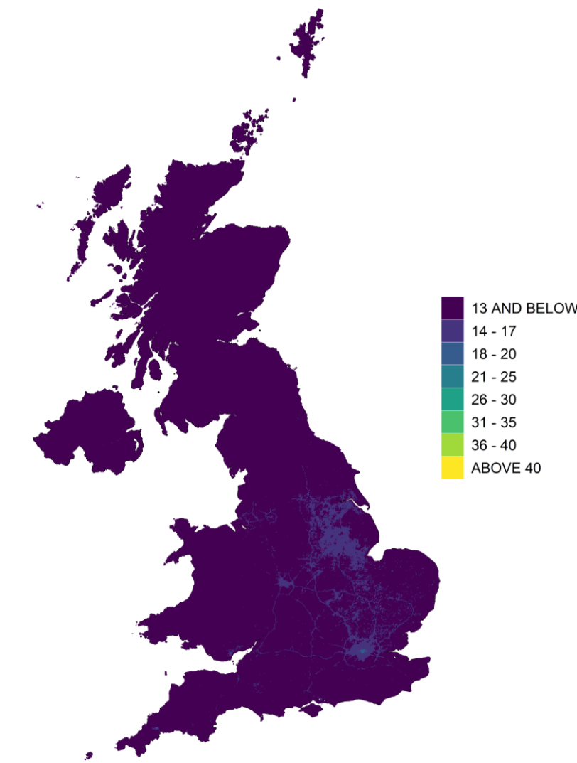
Figure 6.1 - Annual mean background PM 10 concentration, 2021 (µg m -3 , gravimetric)
