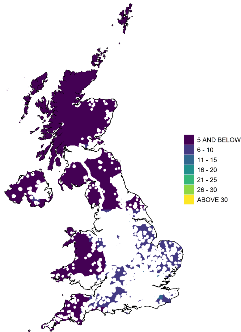
Figure 4.3 - Annual mean map of NO x concentrations for comparison with the NO x vegetation critical level, 2021 ( \mu\text{g m}^{-3} , as NO 2 )
