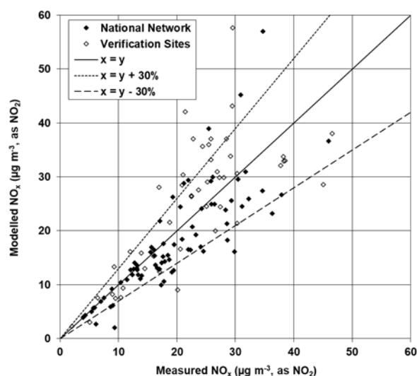
Figure 4.18 - Verification of roadside annual mean NO x model 2021
