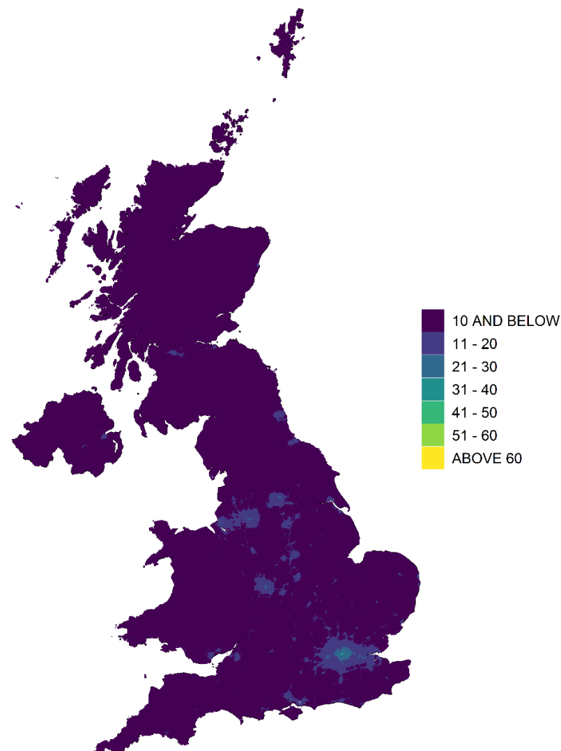
Figure 4.1 - Annual mean background NO 2 concentration, 2021 (µg m -3 )
