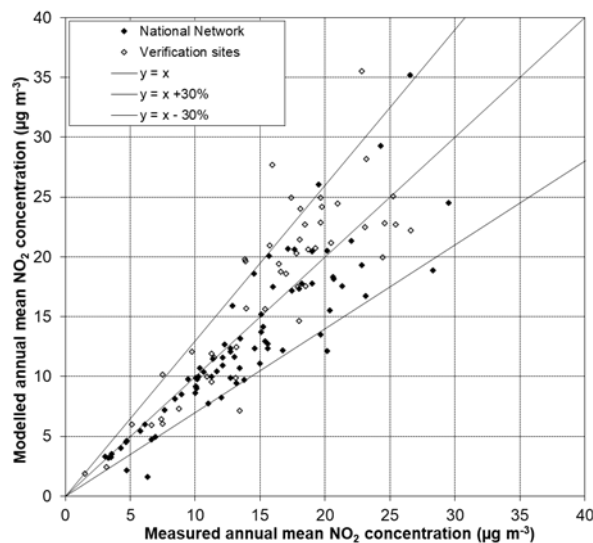
Figure 4.19 - Verification of roadside annual mean NO 2 model 2021
