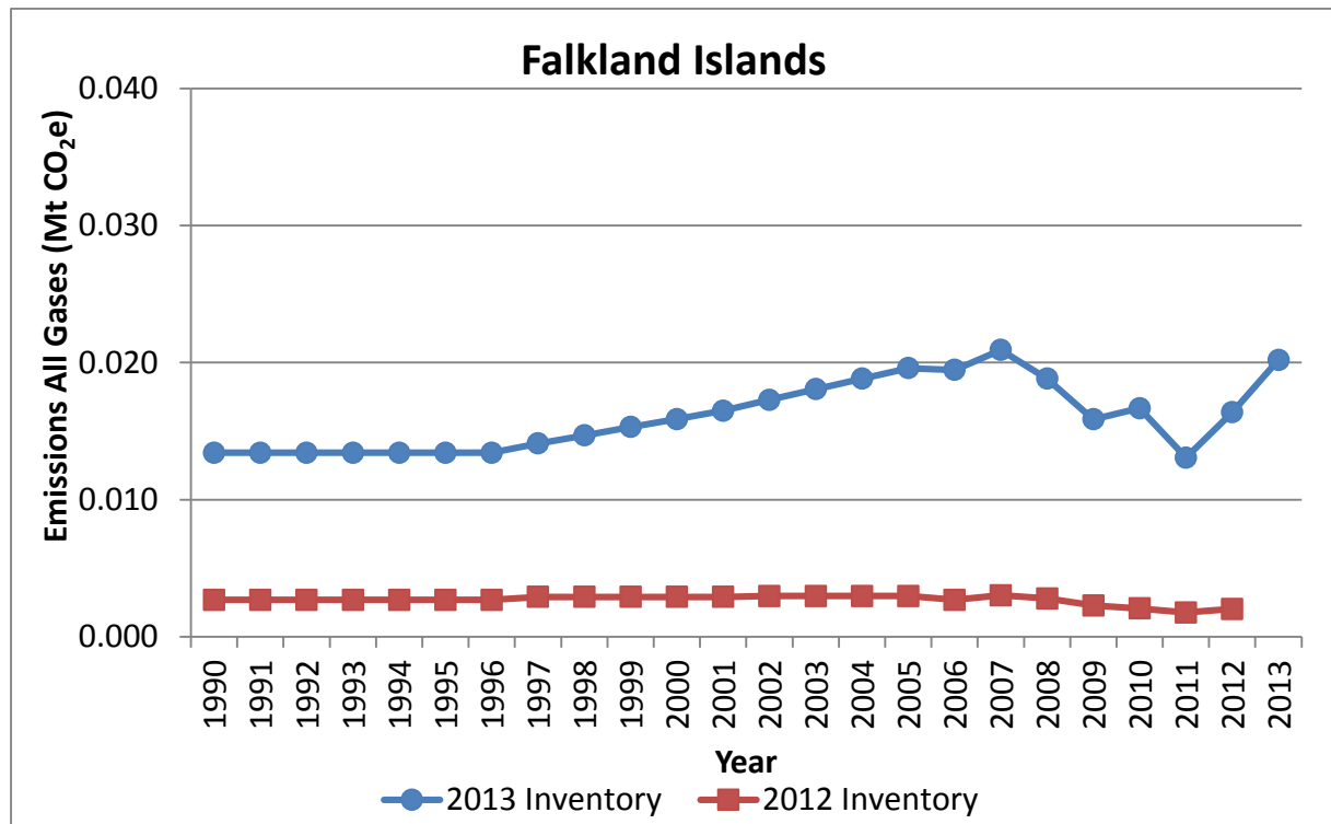
Figure 6.15 LULUCF sector change in net emissions between the 1990-2012 and 1990-2013 inventories for the Falkland Islands
