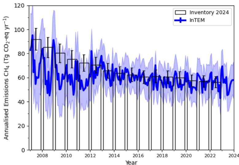
Figure A 6.3 Verification of the UK emission inventory estimates for CH 4 in Tg CO 2 -eq yr -1 from 2007. GHGI estimates are shown in black ( \pm 1\sigma ). InTEM 1-month estimates are shown in blue ( \pm 1\sigma ).
