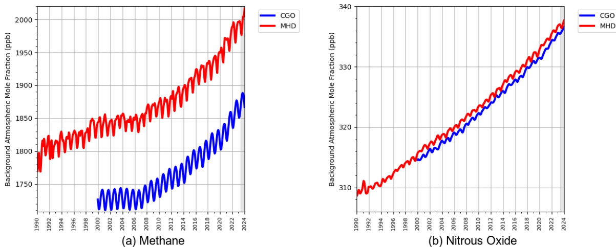
Figure A 6.1 Background Northern Hemisphere monthly concentrations of (a) CH 4 , and (b) N 2 O, estimated from MHD, Ireland observations are shown in red, and background Southern Hemisphere monthly concentrations from CGO, Tasmania are shown in blue. Grey shading represents unratified data.
