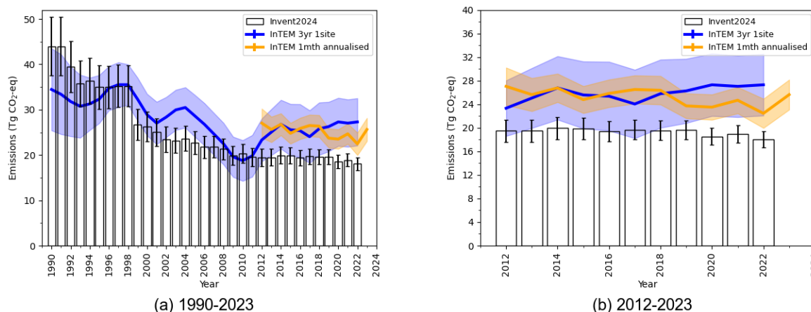
Figure A 6.5 Verification of the UK emission inventory estimates for N 2 O in Tg CO 2 -eq yr -1 (a) from 1990 and (b) from 2012. GHGI estimates are shown in black (±1σ). InTEM 1-site, 3-year estimates are shown in blue (±1σ) and InTEM full network, 1-month, annualised, estimates are in orange (±1σ).
