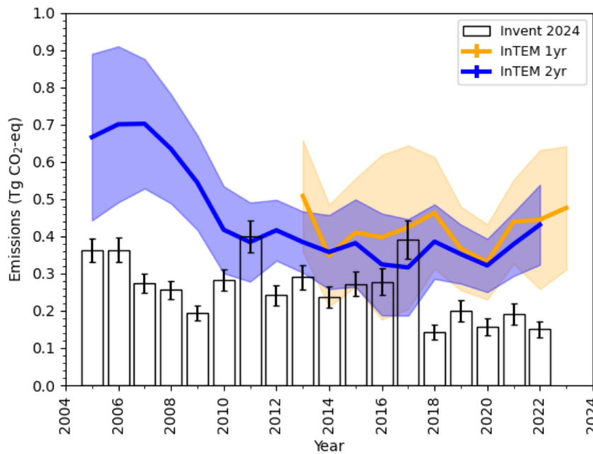
Figure A 6.15 Sum of UK PFC emission estimates (PFC-14, PFC-116, PFC-218, PFC-318) in \text{Tg CO}_2\text{-eq yr}^{-1} from the GHGI (black) and InTEM, annualised 2-year inversion (blue) and 1-year inversion (orange). The uncertainty bounds represent 1\text{-}\sigma .
