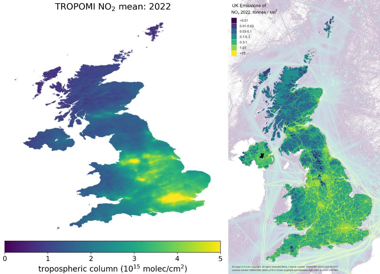
Figure 5-4 NO 2 tropospheric column mean in molecules/cm 2 in 2022 (Left). Total NAEI NO x emissions in tonnes for 2022 (Right). Both maps are plotted in 1x1km
