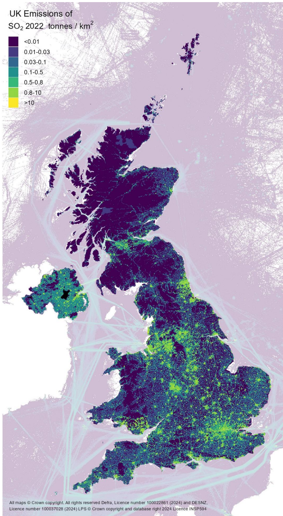
Figure 4-3 UK total SO 2 emissions in 2022.
