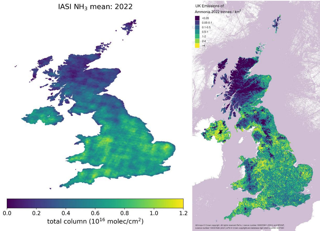
Figure 5-5 NH 3 total column mean in molecules/cm 2 in 2022 (Left). Total NAEI NH 3 emissions in tonnes in 2022 (Right). The IASI map is plotted in 2x2km while the NAEI map is plotted in 1x1km
