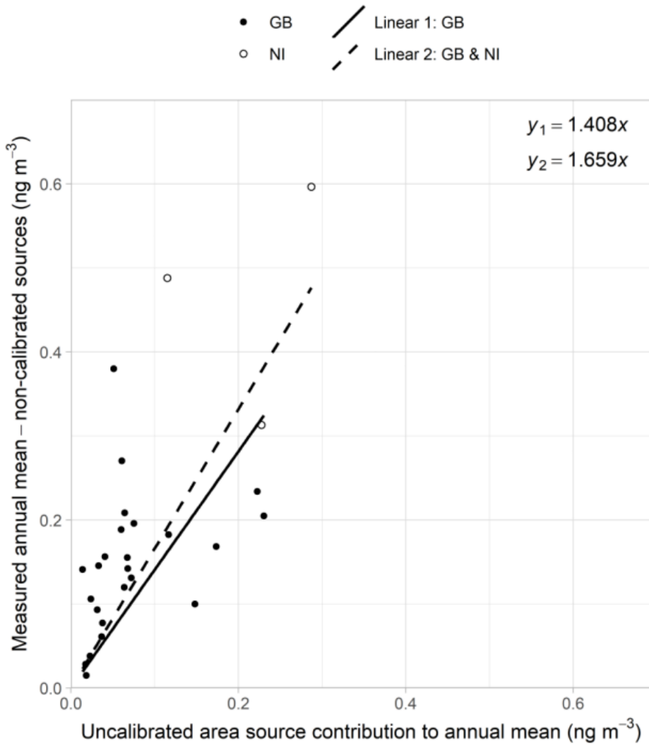
Figure 5-3 Calibration of area source model for B(a)P for the year 2022, where the solid regression line and y_1 refer to Great Britain only, and the dashed line and y_2 refer to Great Britain and Northern Ireland.
