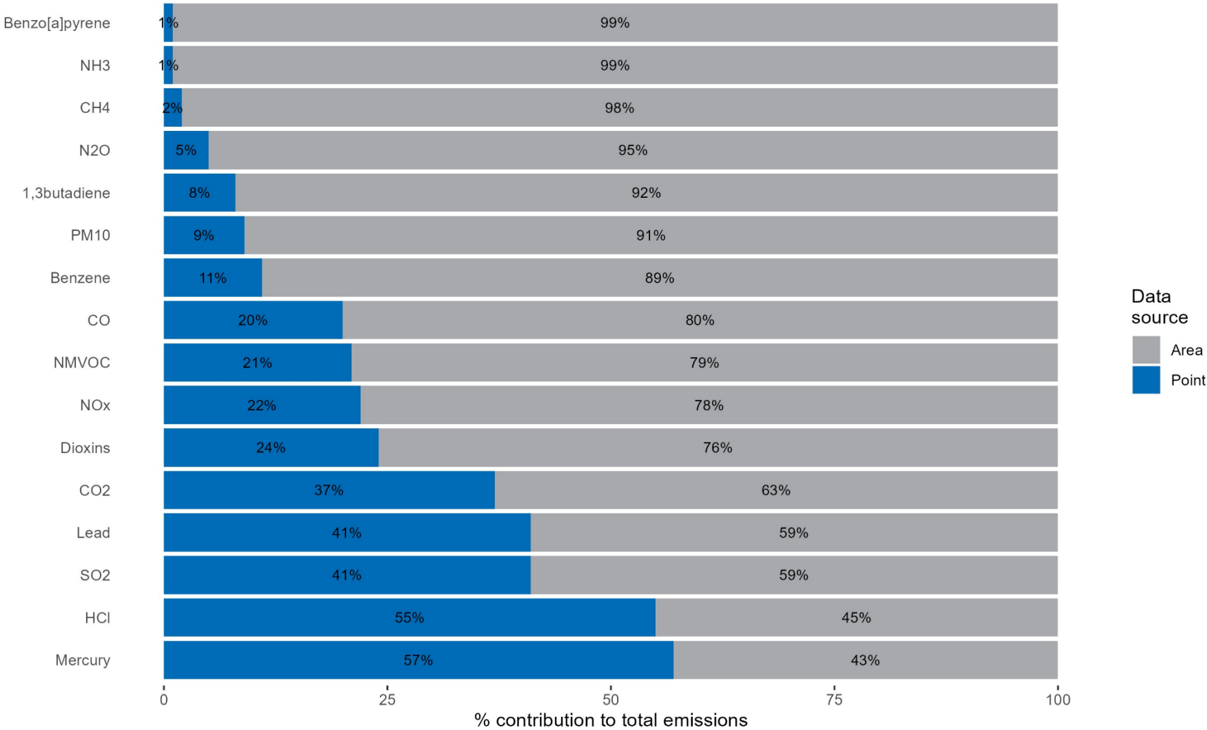
Figure 5-1 Contribution of point sources to mapped emission totals (2022)
