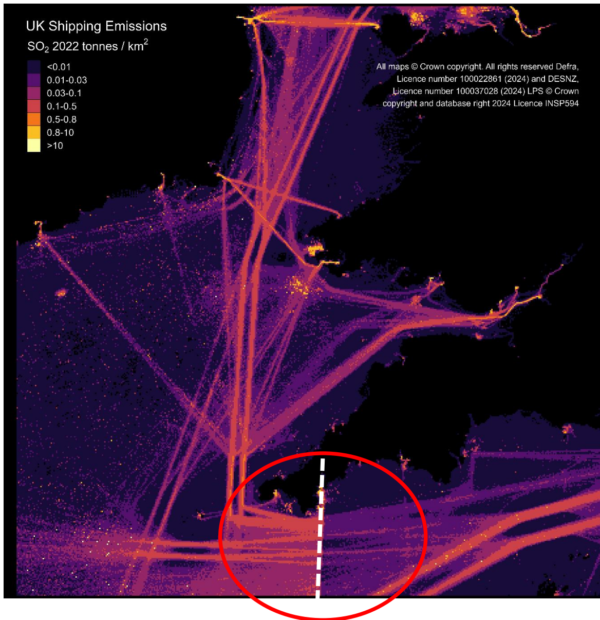
Figure 3-10. SO 2 emissions from all shipping around the south-west of the British Isles. The SECA (Sulphur Emission Control Area) to the east of the dotted white line (bottom centre) can be seen as a reduction in emissions.
