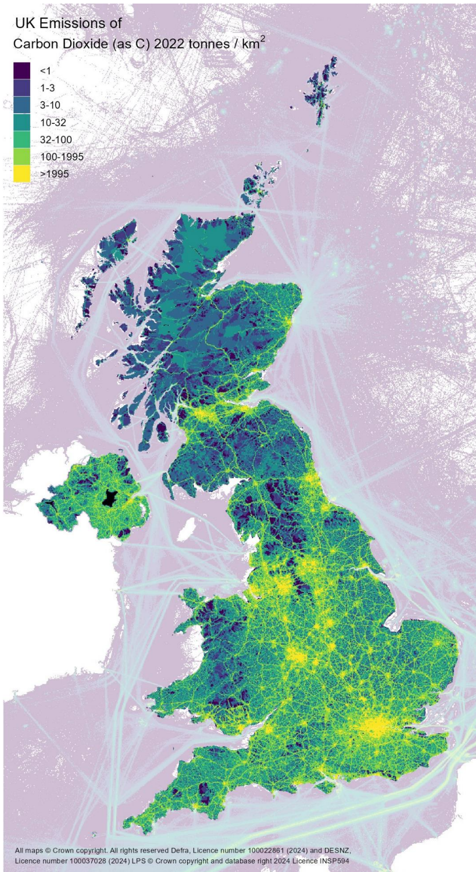
Figure 4-4 UK total CO 2 emissions in 2022 excluding emissions from Land Use Change.
