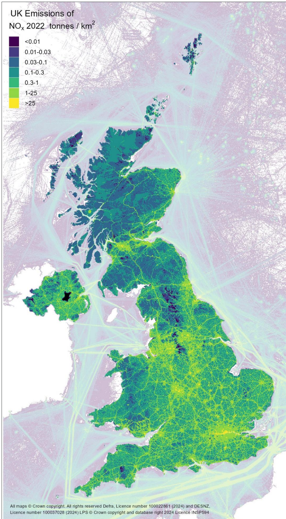
Figure 2-4 UK total NO x emissions in 2022.
