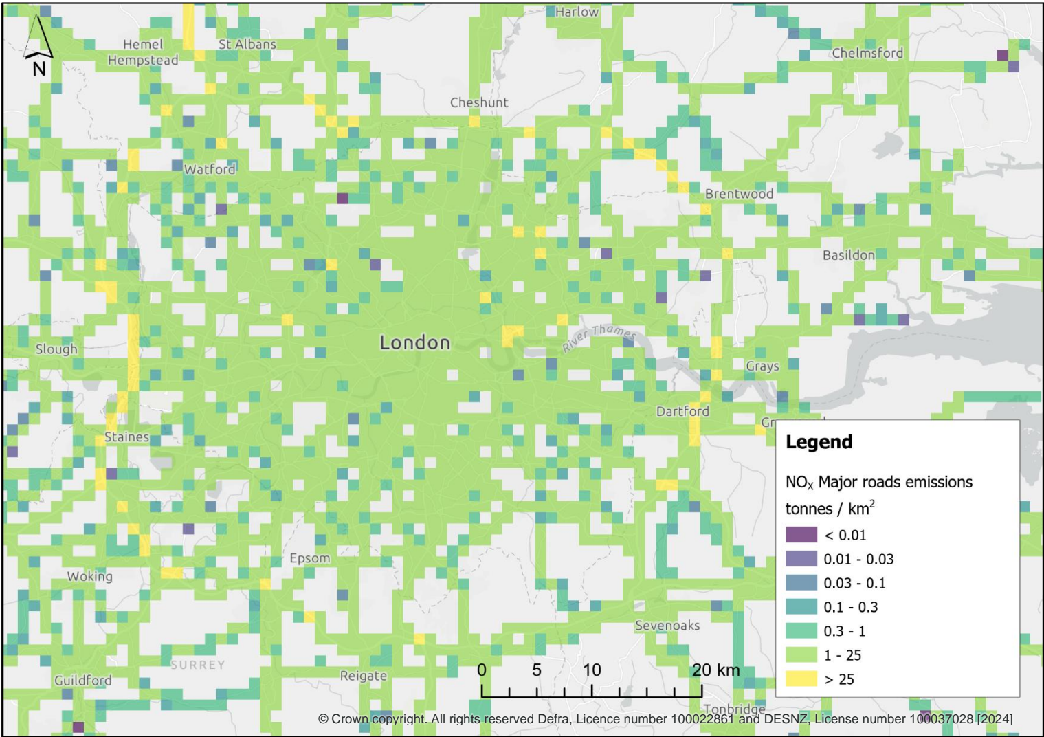
Figure 3-6 2021 NO x road transport emissions on major roads aggregated to 1x1 km resolution.
