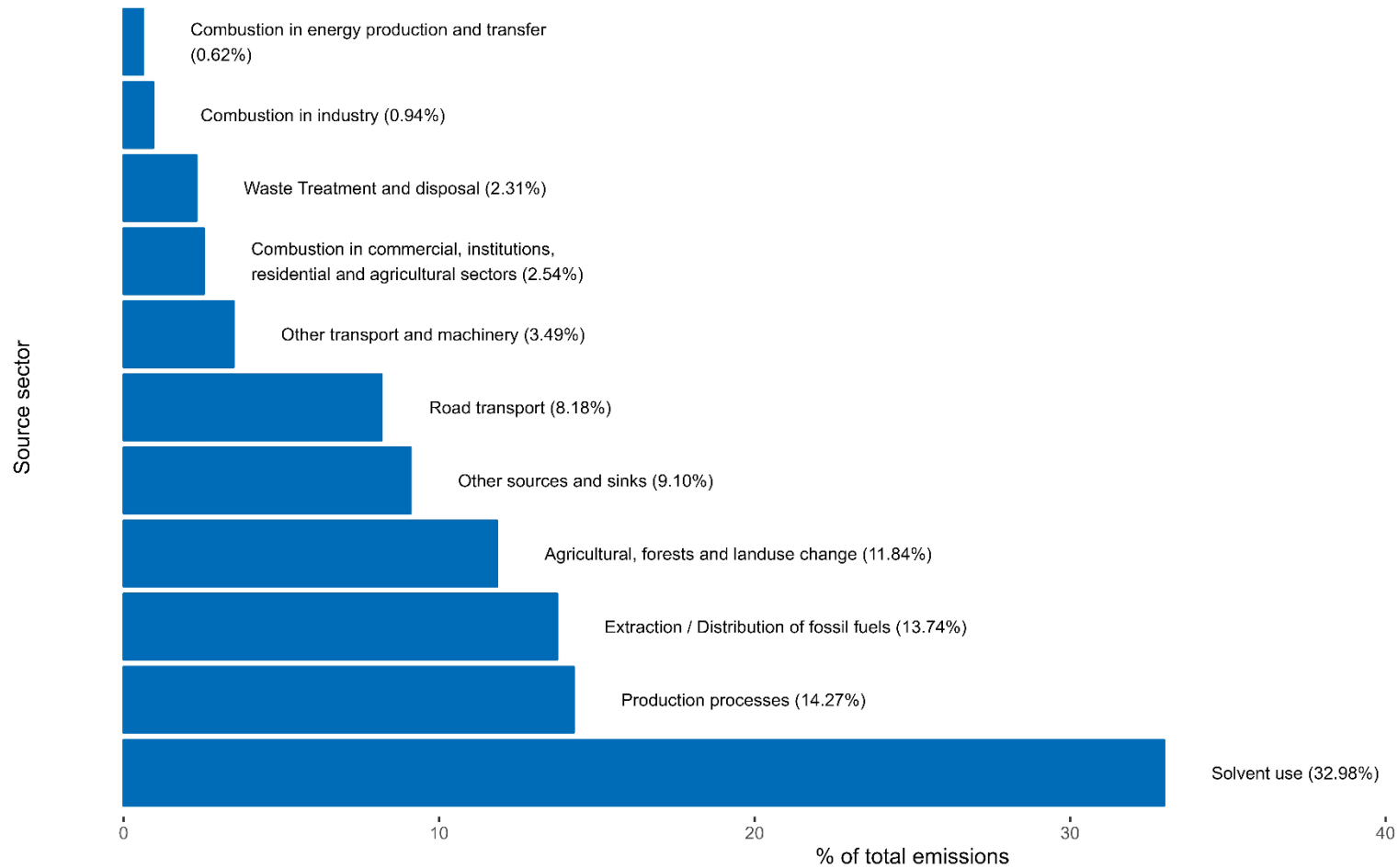
NM VOC Emissions in 2022 by UNECE Source Sector as shown on the NAEI 1x1km maps
