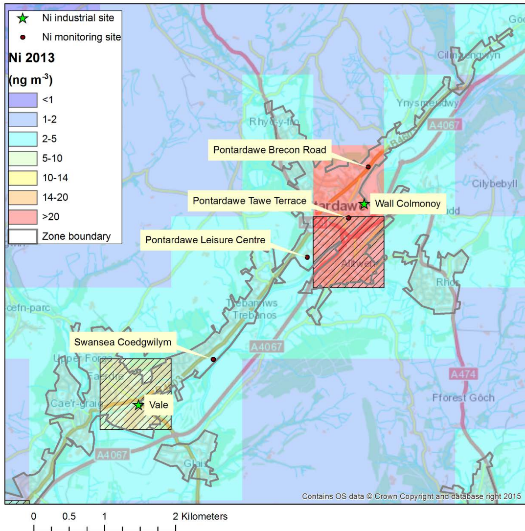
Figure 2 Exceedance situation South Wales [Ni_UK0041_2013_1]. Exceeding grid squares are marked red. Locations of local industrial sites Wall Colmonoy works at Pontardawe and Vale Europe Ltd Clydach refinery and the locations local monitoring stations are also shown. Hatched grid squares are assigned to Swansea Urban Area agglomeration zone UK0027 and do not form part of this exceedance situation.
