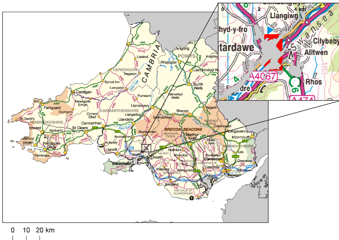
Figure 1. Location of exceedance of the Ni target value on 2013 in the South Wales zone UK0041. Exceeding areas are marked red. The inset map shows the exceedance location within a reduced map extent.
