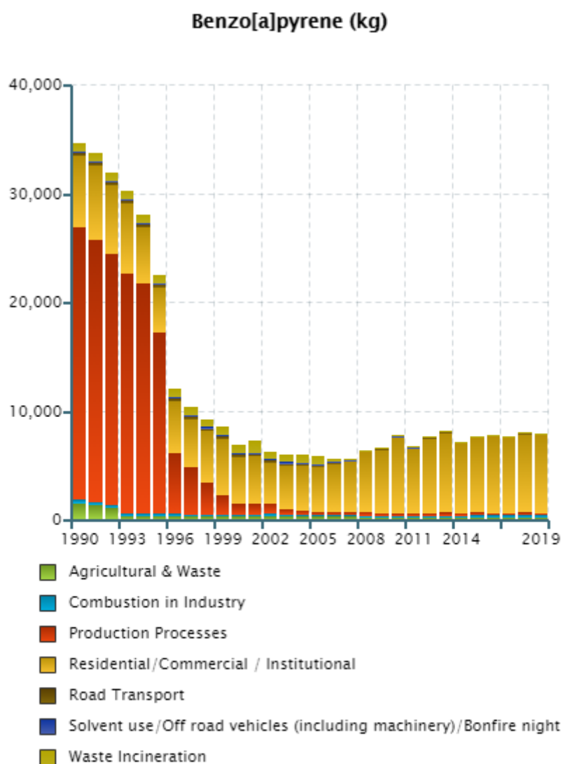
Figure 1. B[a]P emissions by sector (1990-2019)
