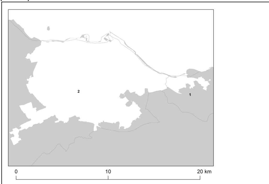
Figure 2. Map showing Local Authorities within the Edinburgh Urban Area agglomeration zone (UK0025).
