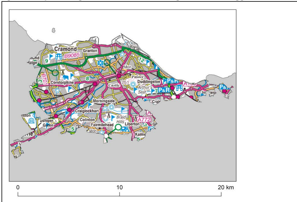
Figure 1. Map showing the extent of the Edinburgh Urban Area agglomeration zone (UK0025).
