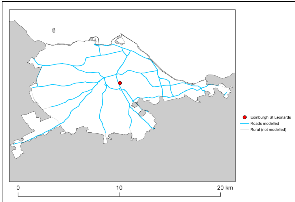
Figure 3. Map showing the location of the NO 2 monitoring sites with valid data in 2008 and roads where concentrations have been modelled within the Edinburgh Urban Area (UK0025) agglomeration zone.
