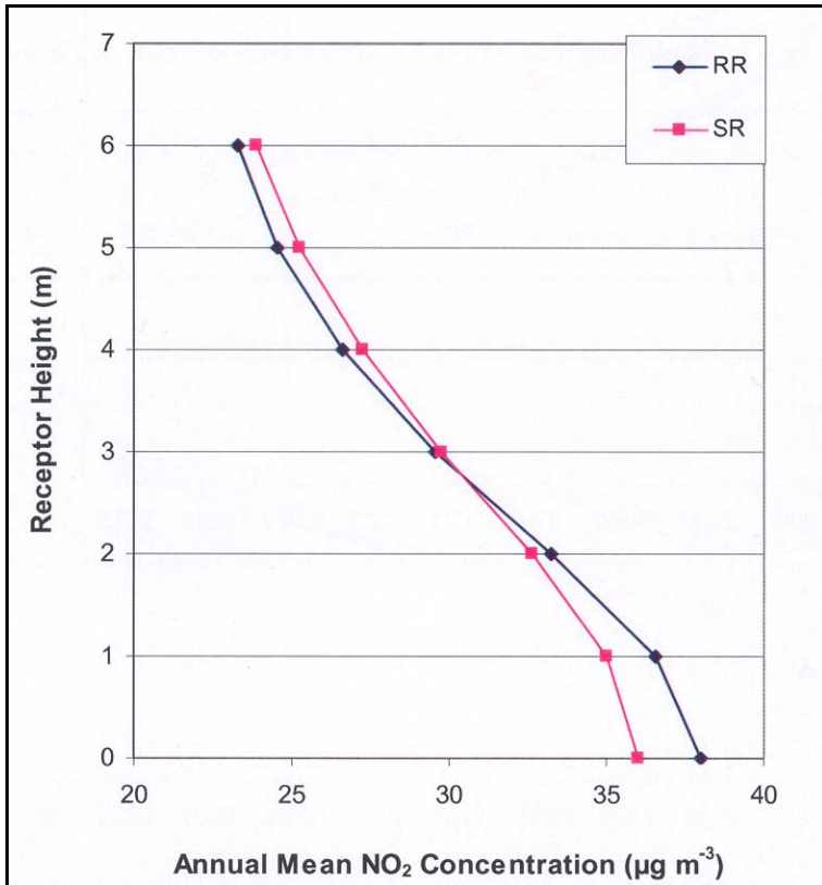
Figure 8. Modelled decrease of NO 2 with height (A5032)
