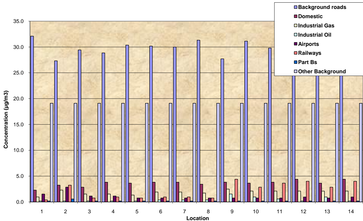
Figure 7. Predicted NO x contributions (µg/m 3 ) for different background sources.
