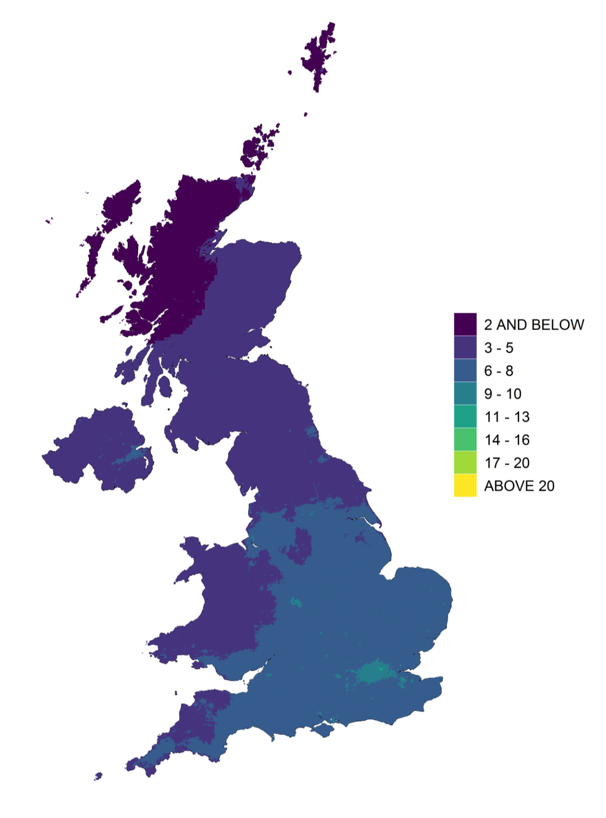
Figure 5-14 Annual Mean Background PM 2.5 Concentration, 2020 (µg m -3 )
