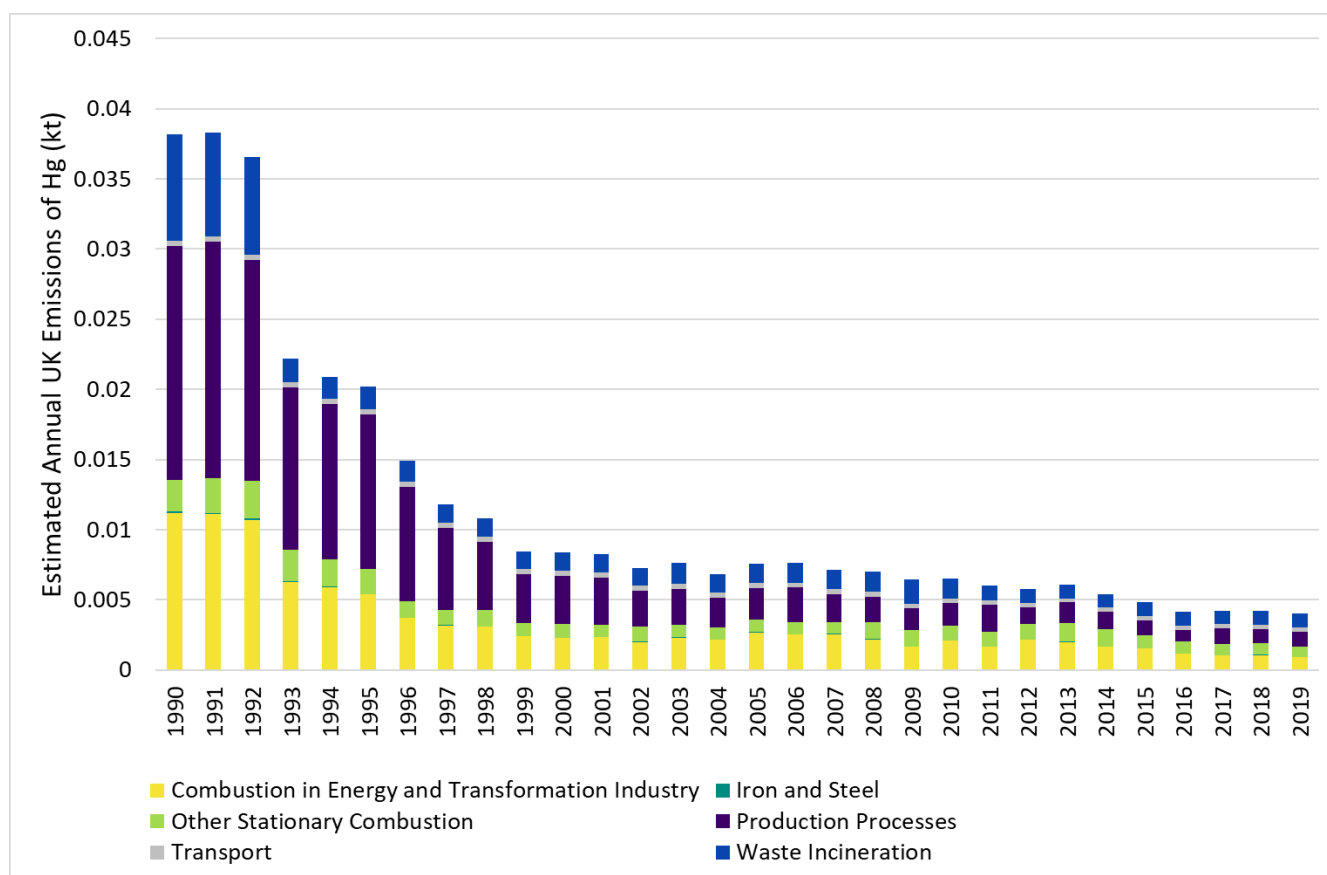
Figure 5-47 Estimated Annual UK Emissions of Hg, 1990 - 2019 (source: NAEI 2019)
