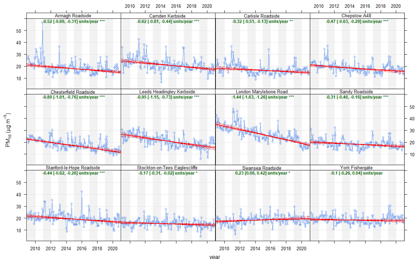
Figure 5-11 De-seasonalised Trends in Ambient PM 10 , 12 Long-Running Urban Traffic AURN Sites 2009 – 2020
