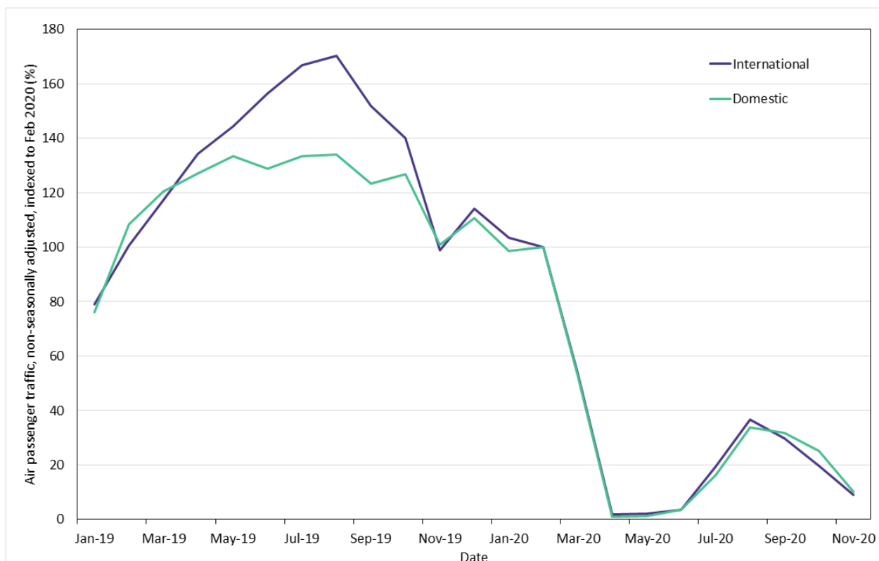
Figure 6-5 International and domestic air passenger traffic, non-seasonally adjusted, indexed to February 2020 (i.e. February 2020 = 100%). Source: Civil Aviation Authority. Data accessed from https://www.ons.gov.uk/ .
