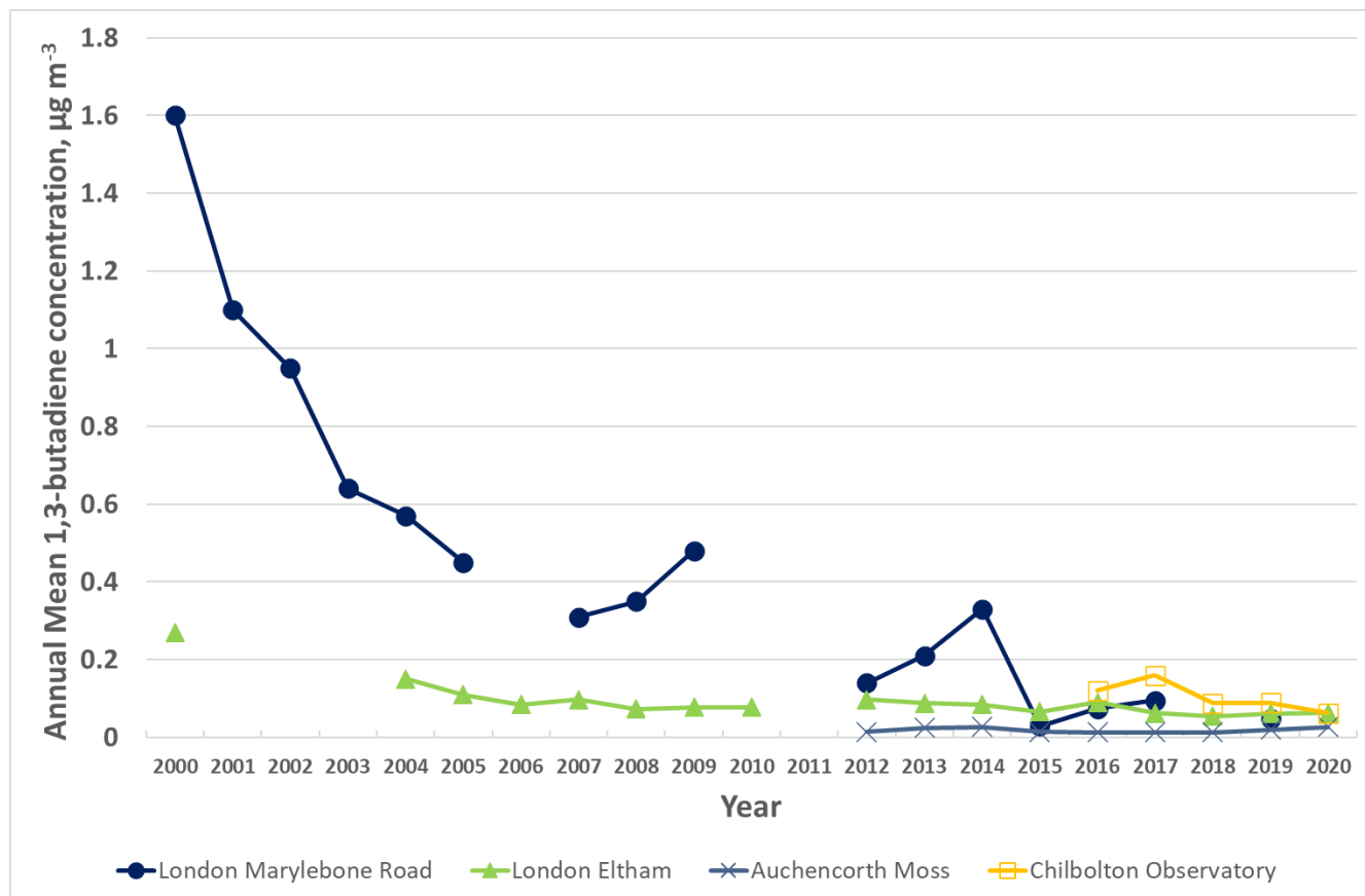
Figure 5-33 Time Series Graph of 1,3-Butadiene Concentration, 2000-2020
