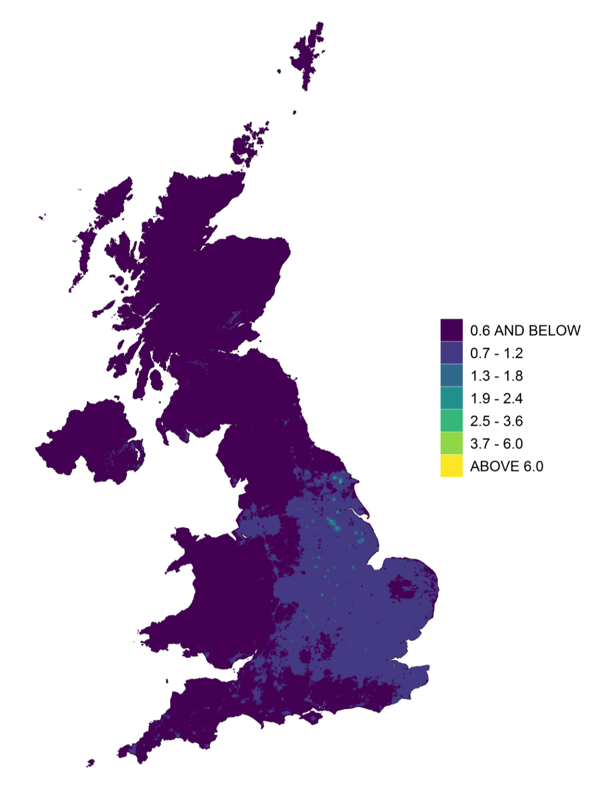
Figure 5-36 Annual Mean Background Arsenic Concentration, 2020 (ng m -3 )
