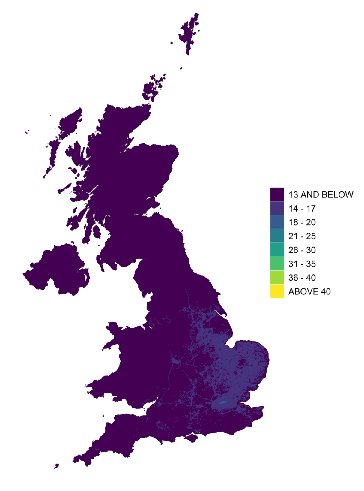
Figure 5-7 Annual Mean Background PM 10 Concentration, 2020 (µg m -3 )
