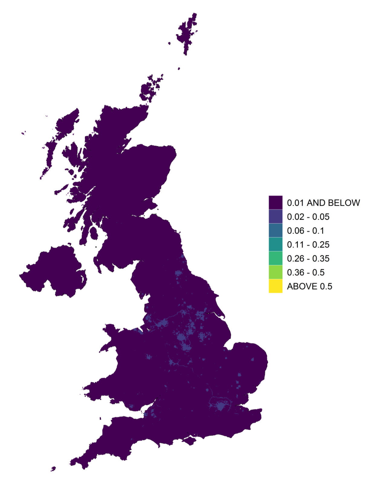
Figure 5-35 Annual Mean Background Lead Concentration, 2020 ( \mu\text{g m}^{-3} )
