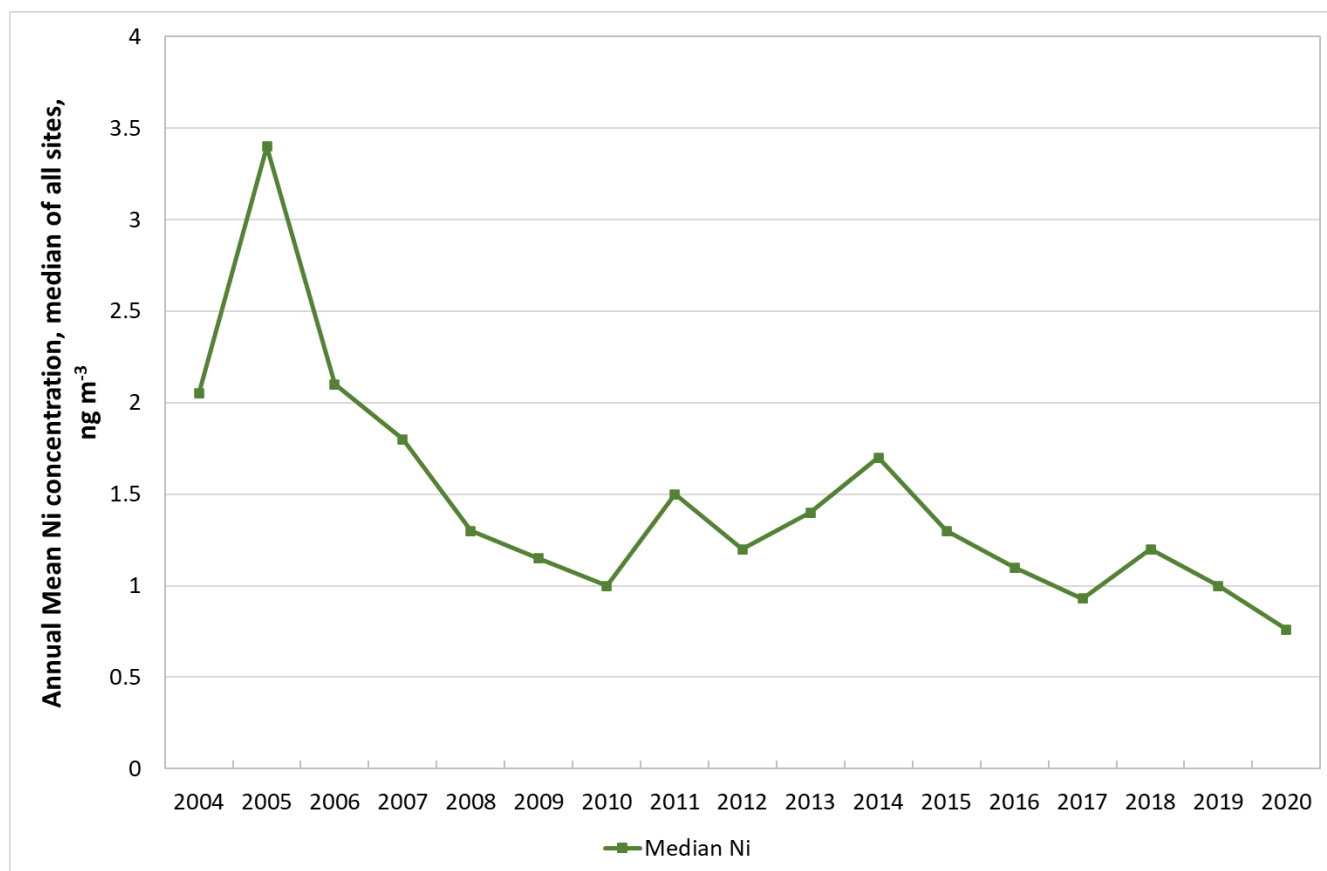
Figure 5-45 Ambient Concentrations of Ni in PM 10 , 2004 – 2020
