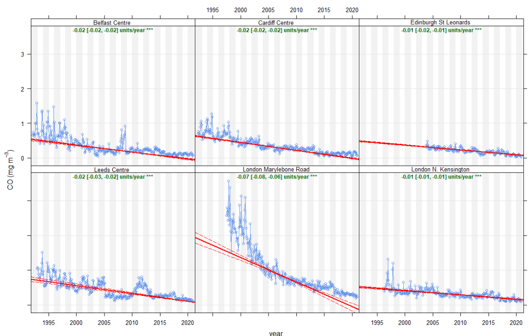
Figure 5-27 De-seasonalised Trends in CO Concentration, 6 Long-Running AURN Sites 1992-2020
