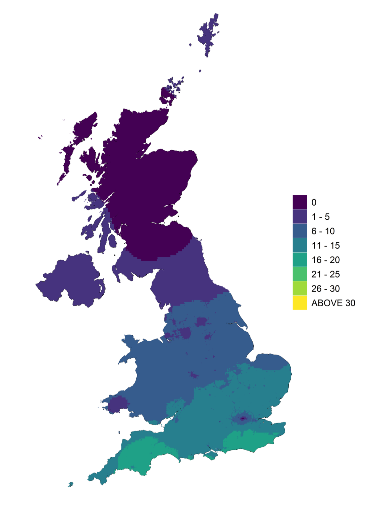
Figure 5-19 Days with O 3 Concentration > 120 µg m -3 , 2020
