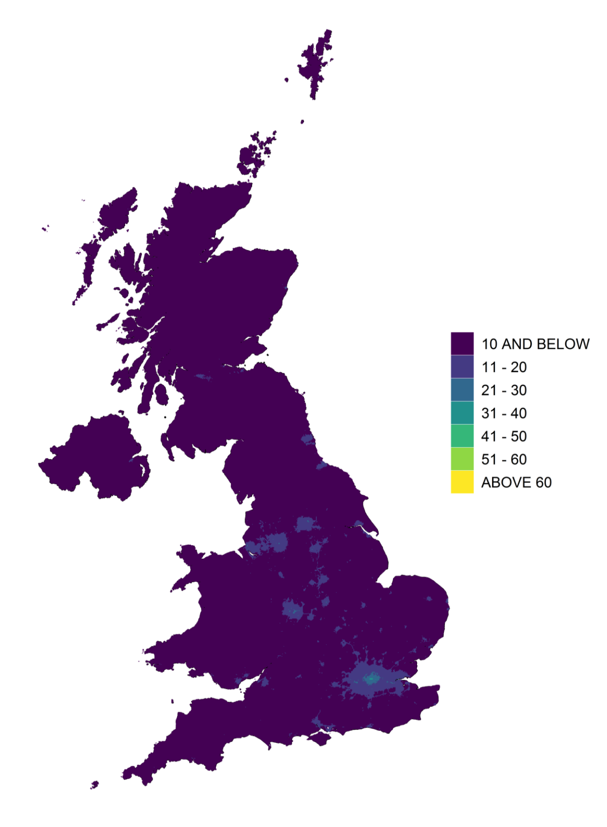
Figure 5-2 Annual Mean Background NO 2 Concentration, 2020 (µg m -3 )
