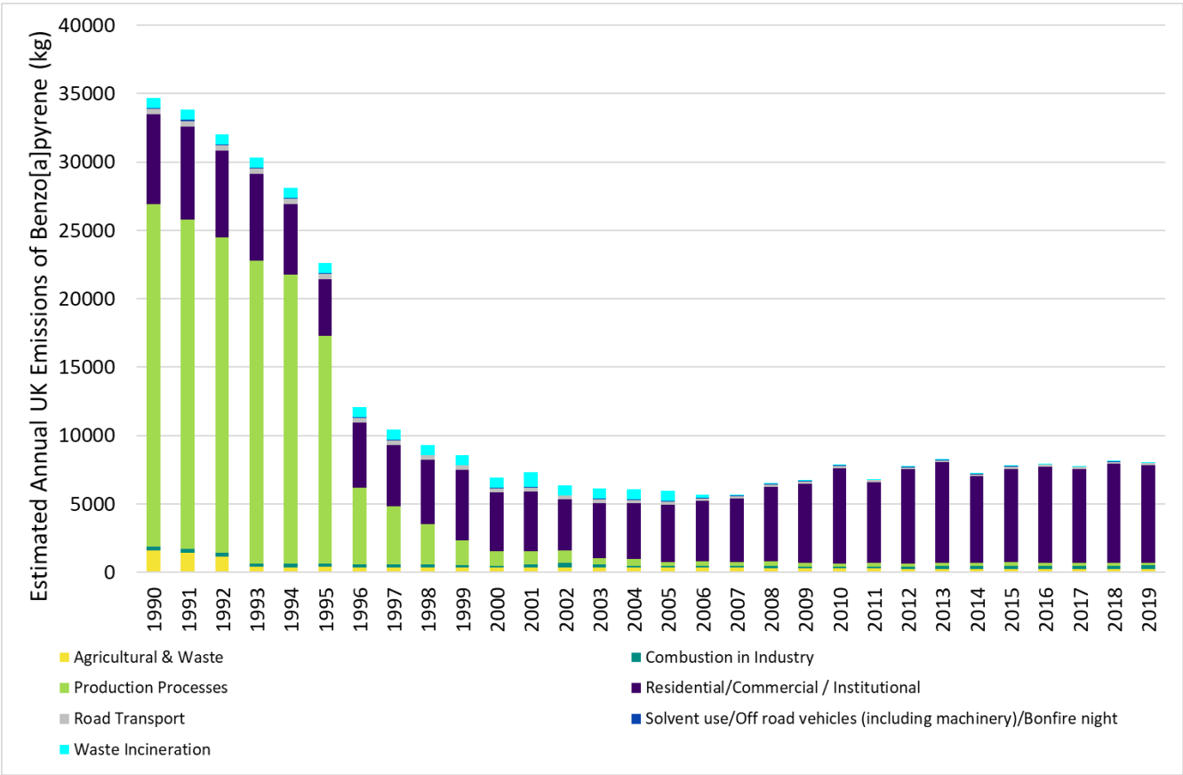
Figure 5-50 Estimated Annual UK Emissions of Benzo[a]pyrene (kg), 1990 – 2019 (source: NAEI)
