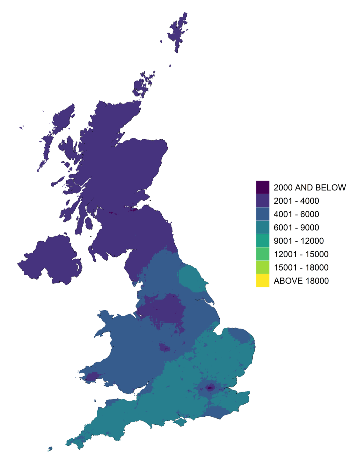
Figure 5-20 Average AOT40, 2016-2020 ( \mu\text{g m}^{-3}\cdot\text{hours} )
