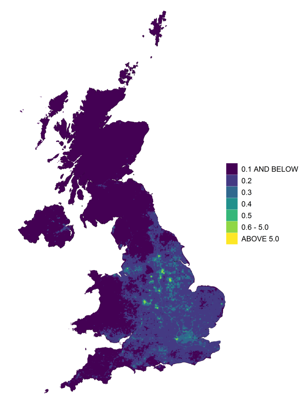
Figure 5-37 Annual Mean Background Cadmium Concentration, 2020 (ng m -3 )
