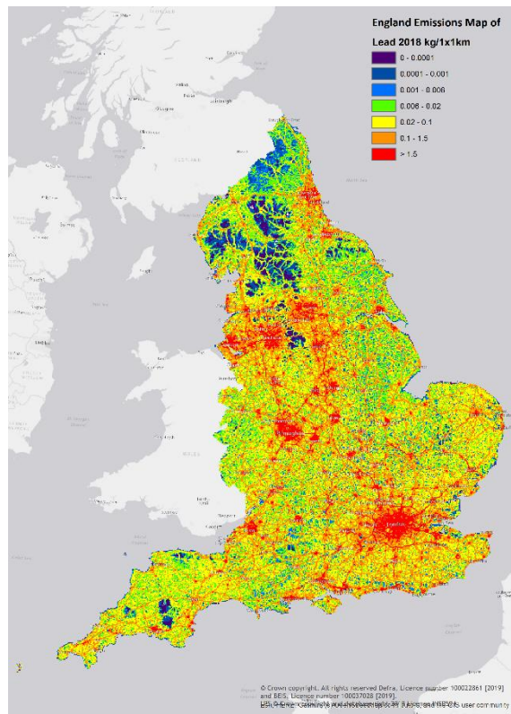
Figure 16 – Lead Emissions in England, 2018
