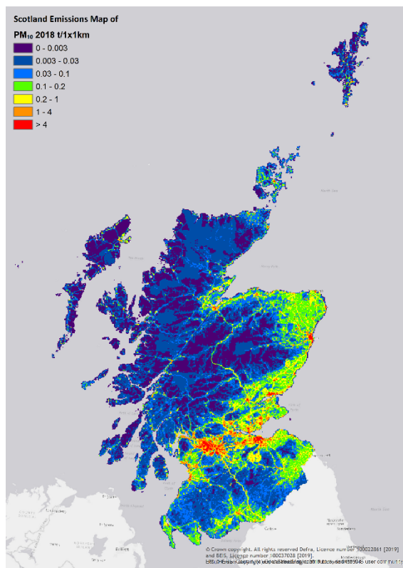
Figure 31 – PM 10 Emissions in Scotland, 2018
