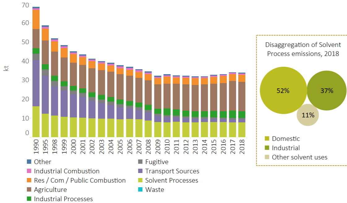
Figure 56 – NMVOC Emissions in Northern Ireland
