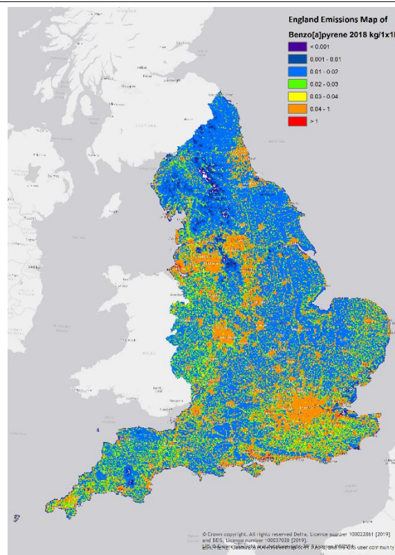
Figure 72 B[a]p Emissions in England, 2018
