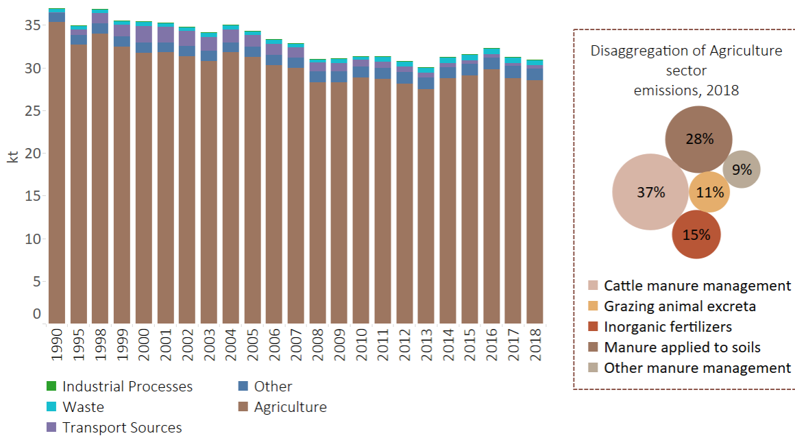
Figure 19 – Ammonia Emissions in Scotland
