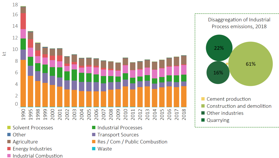
Figure 57 – PM 10 Emissions in Northern Ireland
