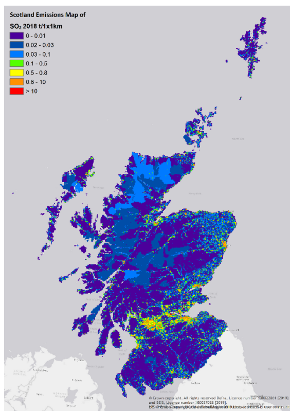
Figure 34 – Sulphur Dioxide Emissions in Scotland, 2018
