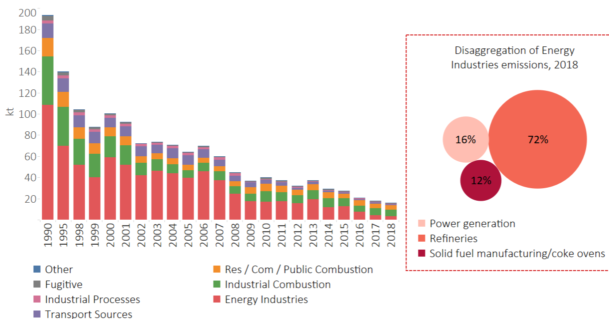
Figure 42 – Sulphur Dioxide Emissions in Wales
