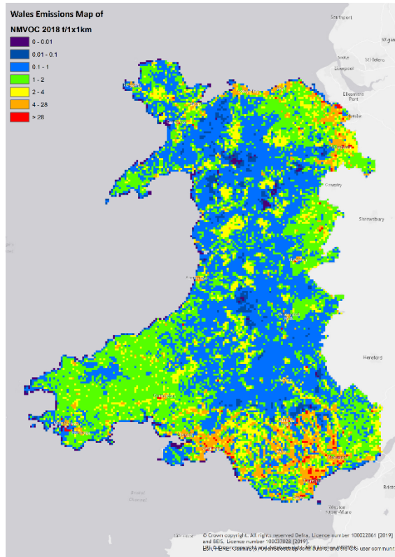
Figure 47 – NMVOC Emissions in Wales, 2018
