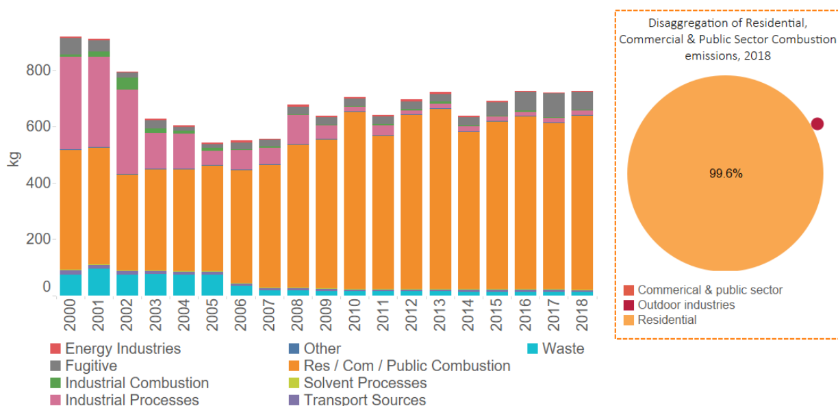
Figure 78 B[a]p Emissions in Wales
