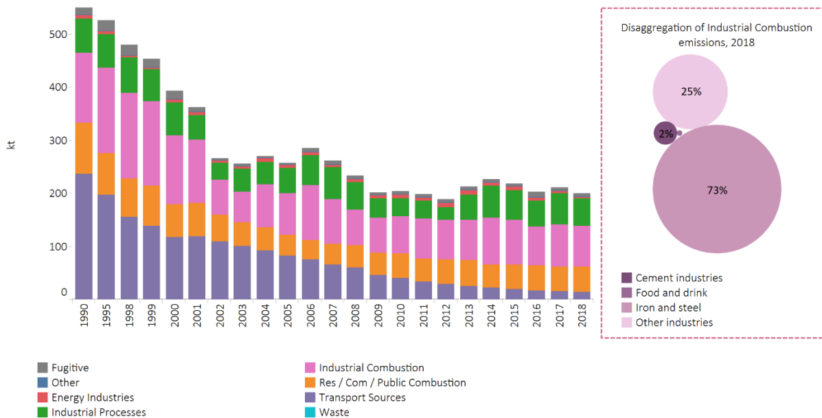
Figure 37 – Carbon Monoxide Emissions in Wales
