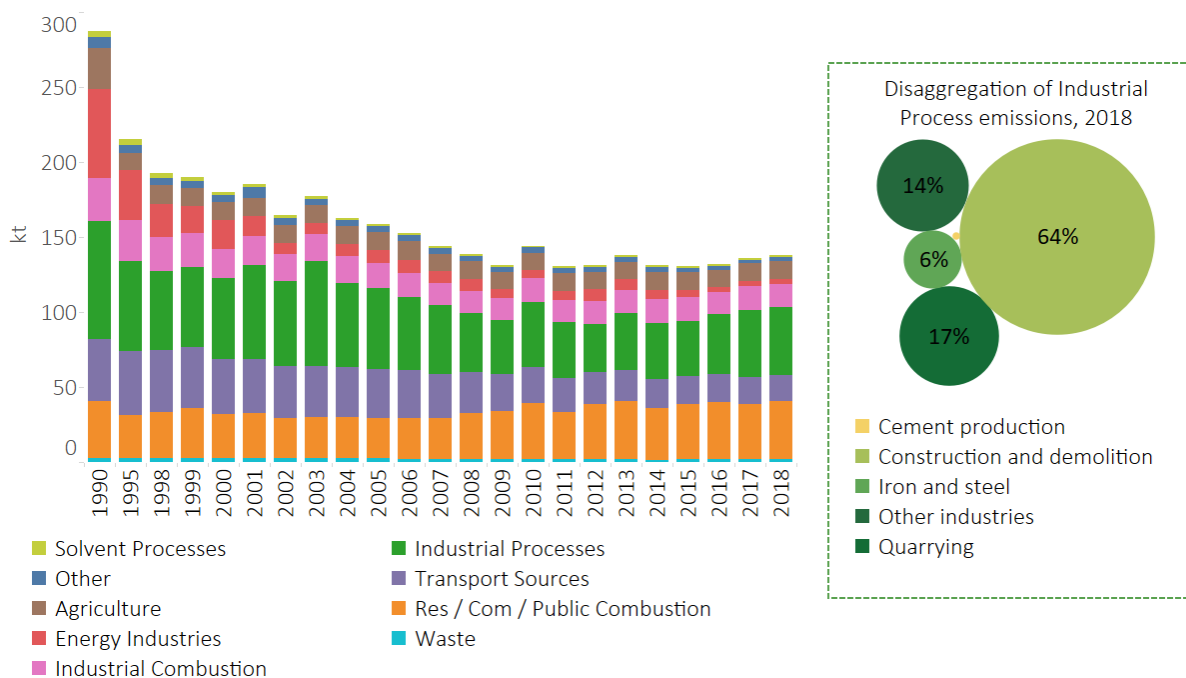
Figure 6 – PM 10 Emissions in England
