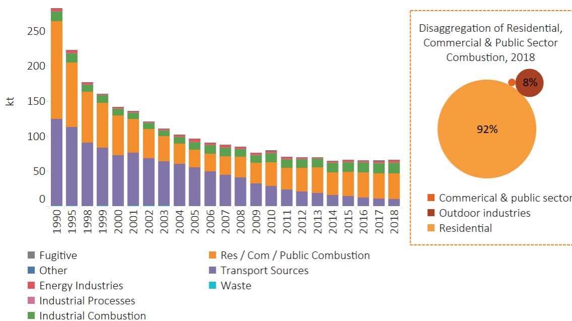
Figure 54 – Carbon Monoxide Emissions in Northern Ireland
