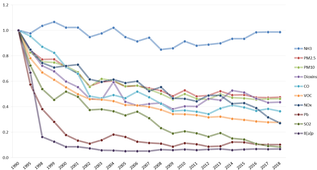
Figure 35 – Wales normalised trends for all pollutants
