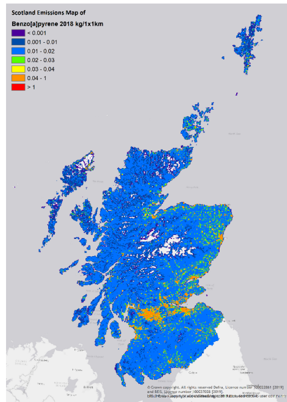
Figure 76 B[a]p Emissions in Scotland, 2018
