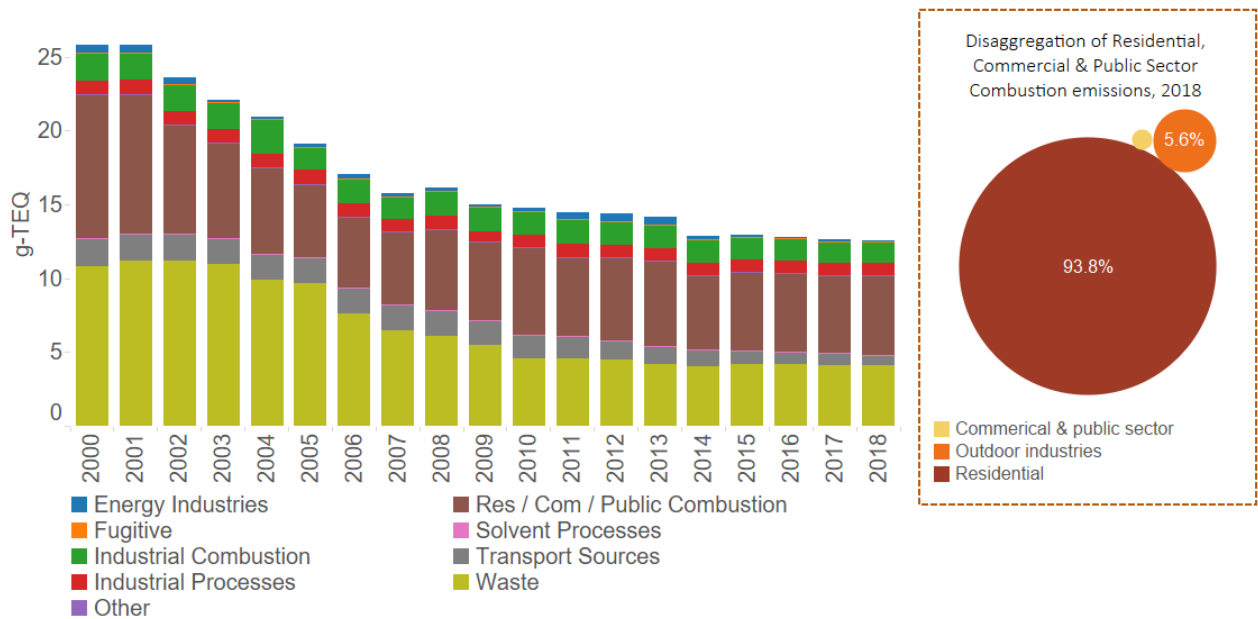
Figure 73 Dioxins Emissions in Scotland
