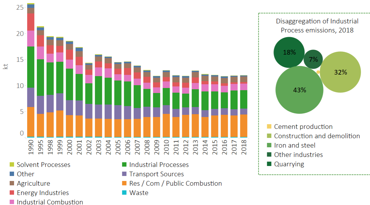
Figure 40 – PM 10 Emissions in Wales
