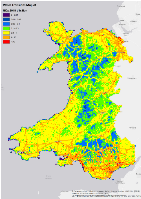
Figure 46 – Nitrogen Oxides Emissions in Wales, 2018
