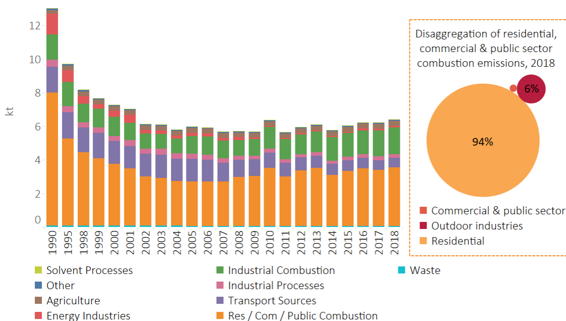
Figure 58 - PM 2.5 Emissions in Northern Ireland
