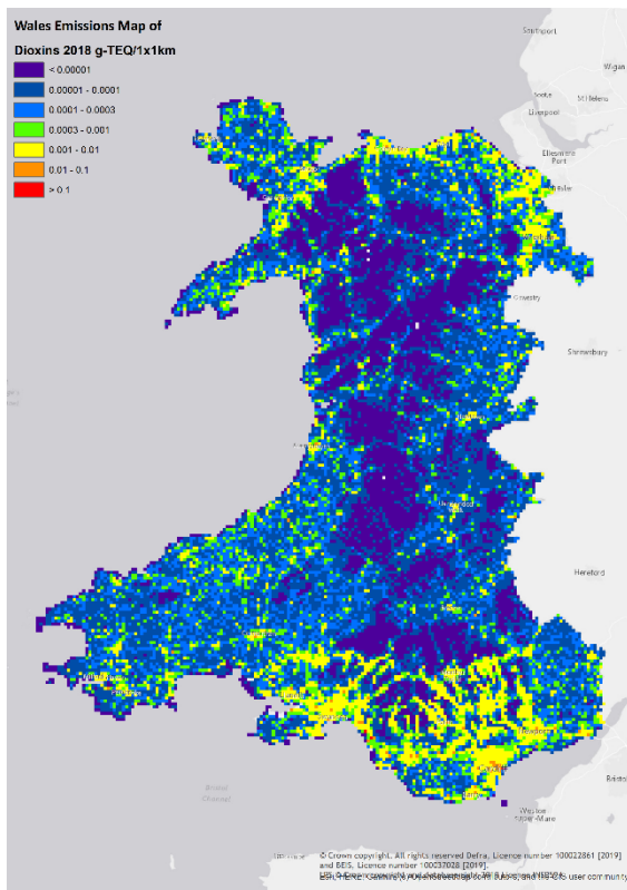
Figure 79 Dioxin Emissions in Wales, 2018
