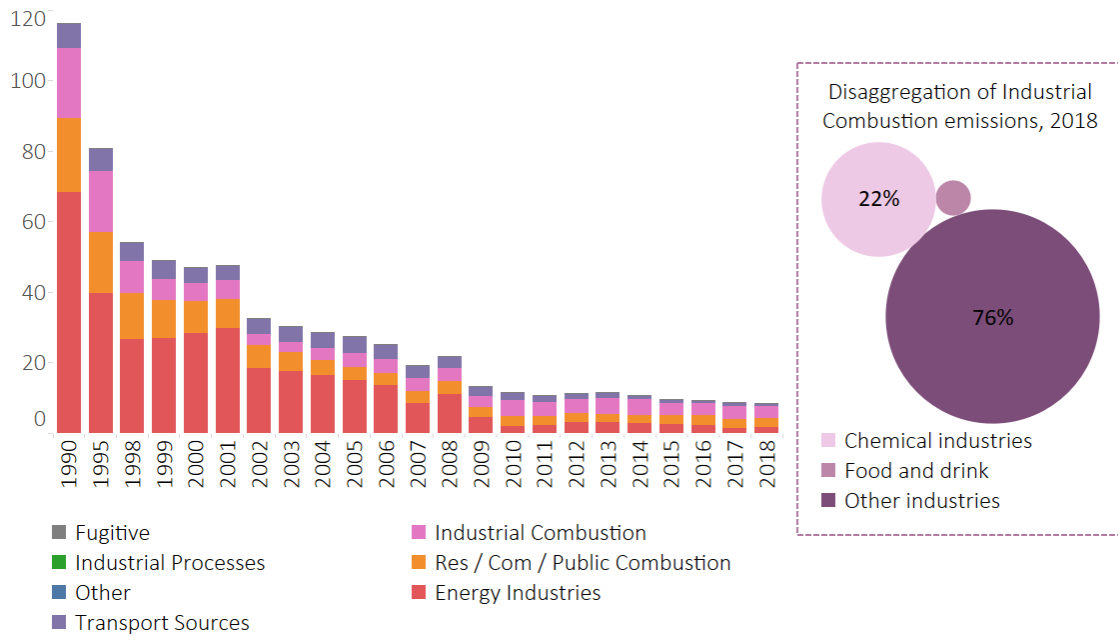
Figure 59 – Sulphur Dioxide Emissions in Northern Ireland
