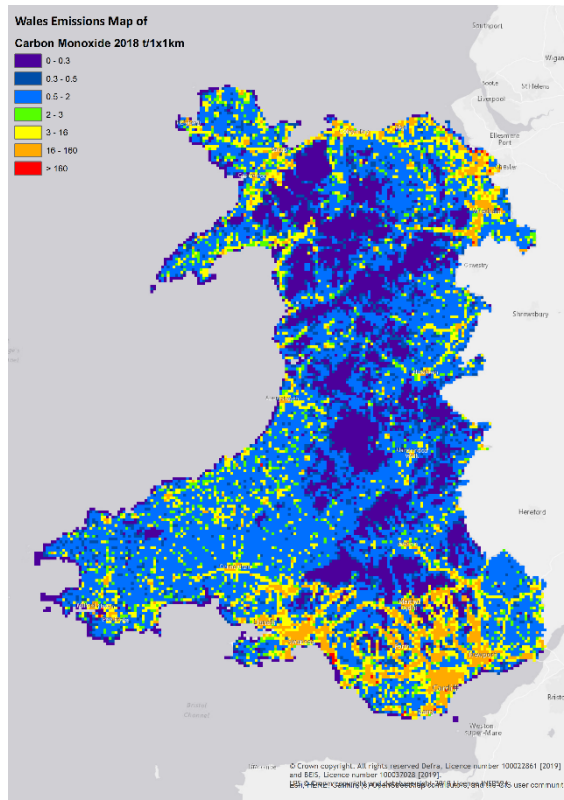
Figure 45 – Carbon Monoxide Emissions in Wales, 2018
