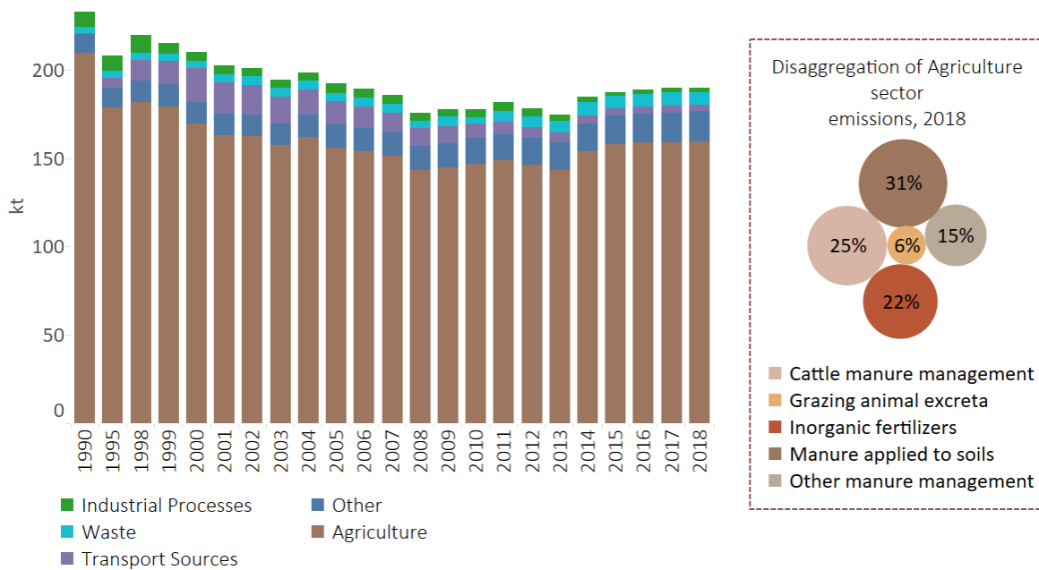
Figure 2 – Ammonia Emissions in England
