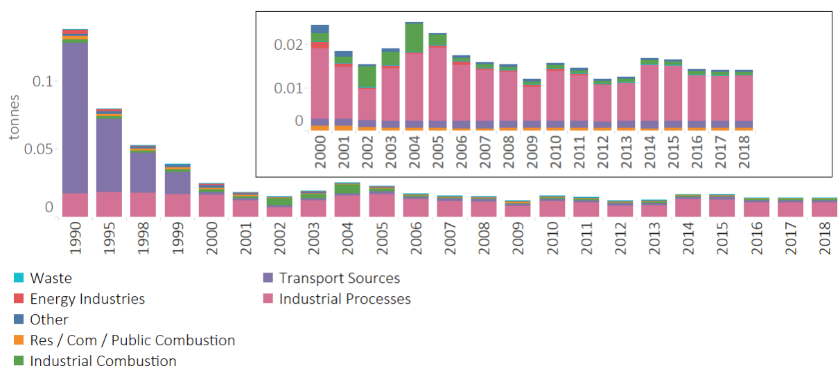
Figure 43 – Lead Emissions in Wales
