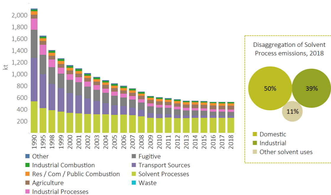
Figure 5 – NMVOC Emissions in England
