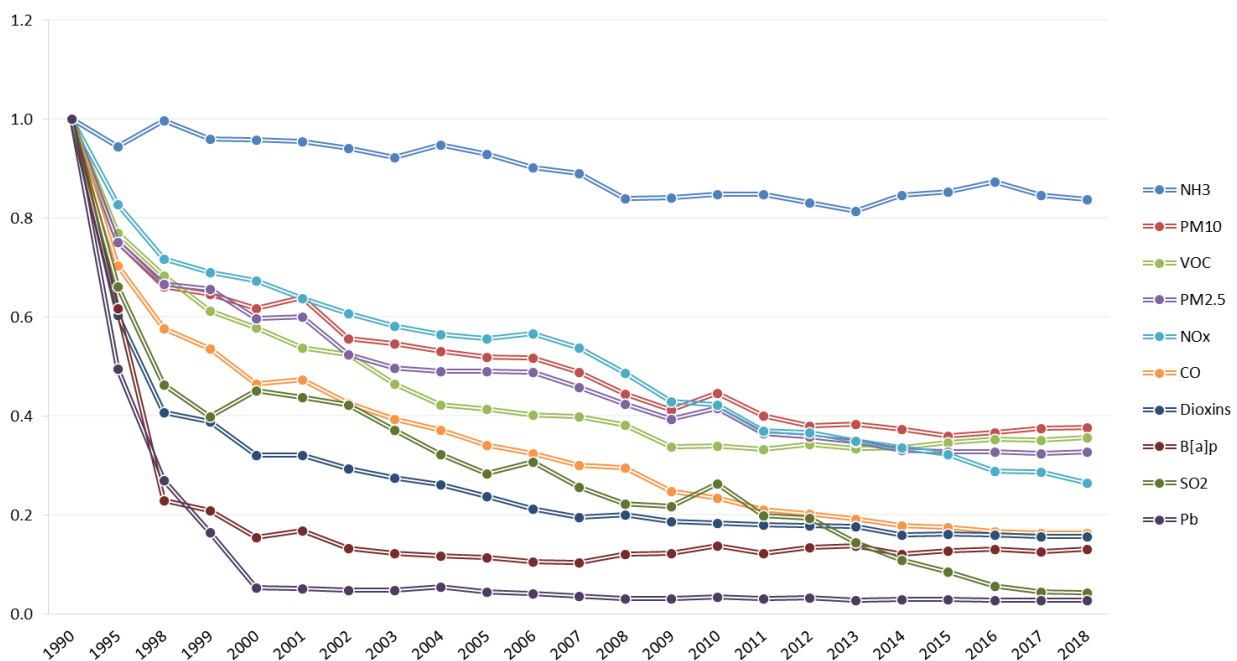
Figure 18 - Scotland normalised trends for all pollutants
