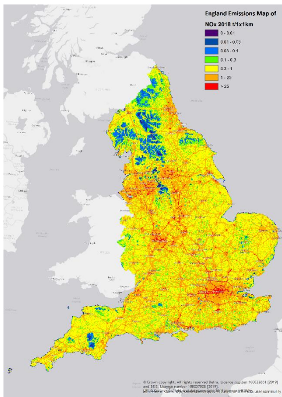
Figure 12 – Nitrogen Oxides Emissions in England, 2018
