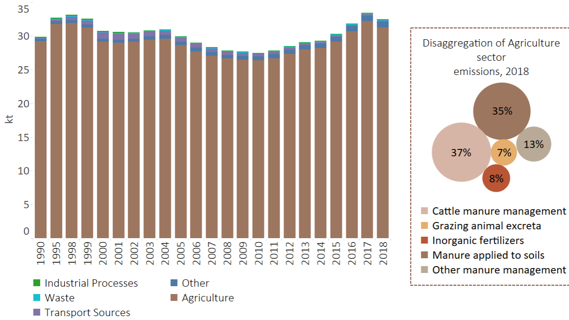
Figure 53 – Ammonia Emissions in Northern Ireland
