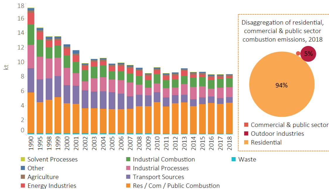
Figure 41 – PM 2.5 Emissions in Wales 3
