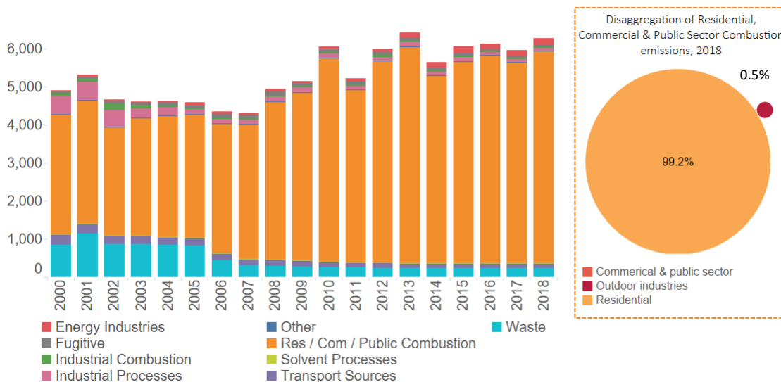
Figure 70 B[a]p emissions in England
