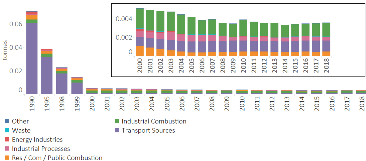
Figure 60 – Lead Emissions in Northern Ireland
