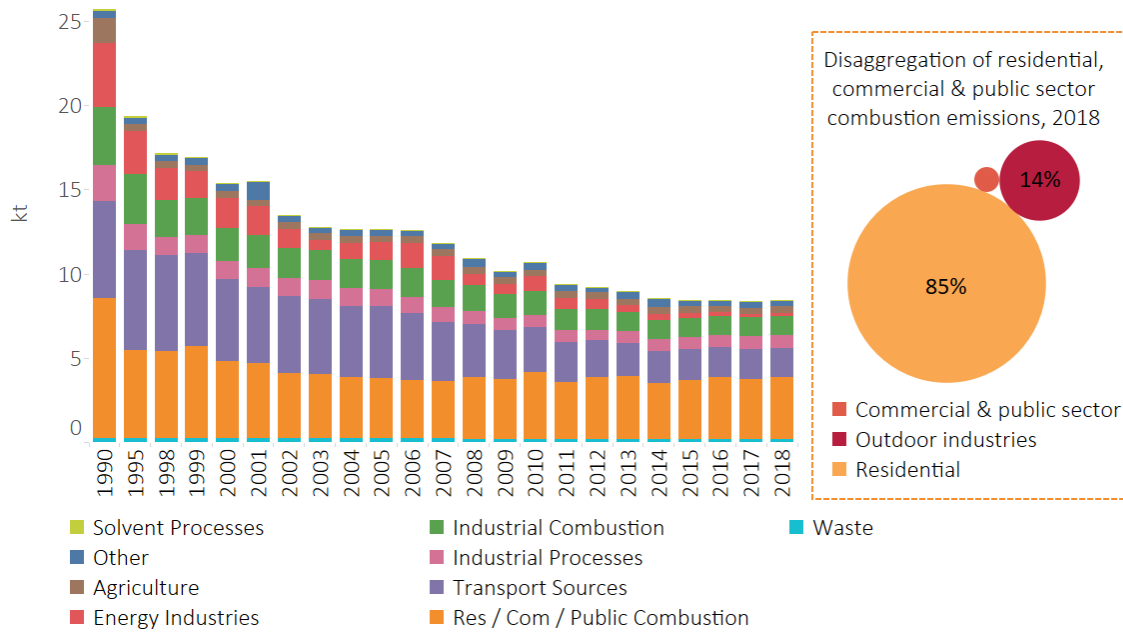
Figure 24 – PM 2.5 Emissions in Scotland 2
