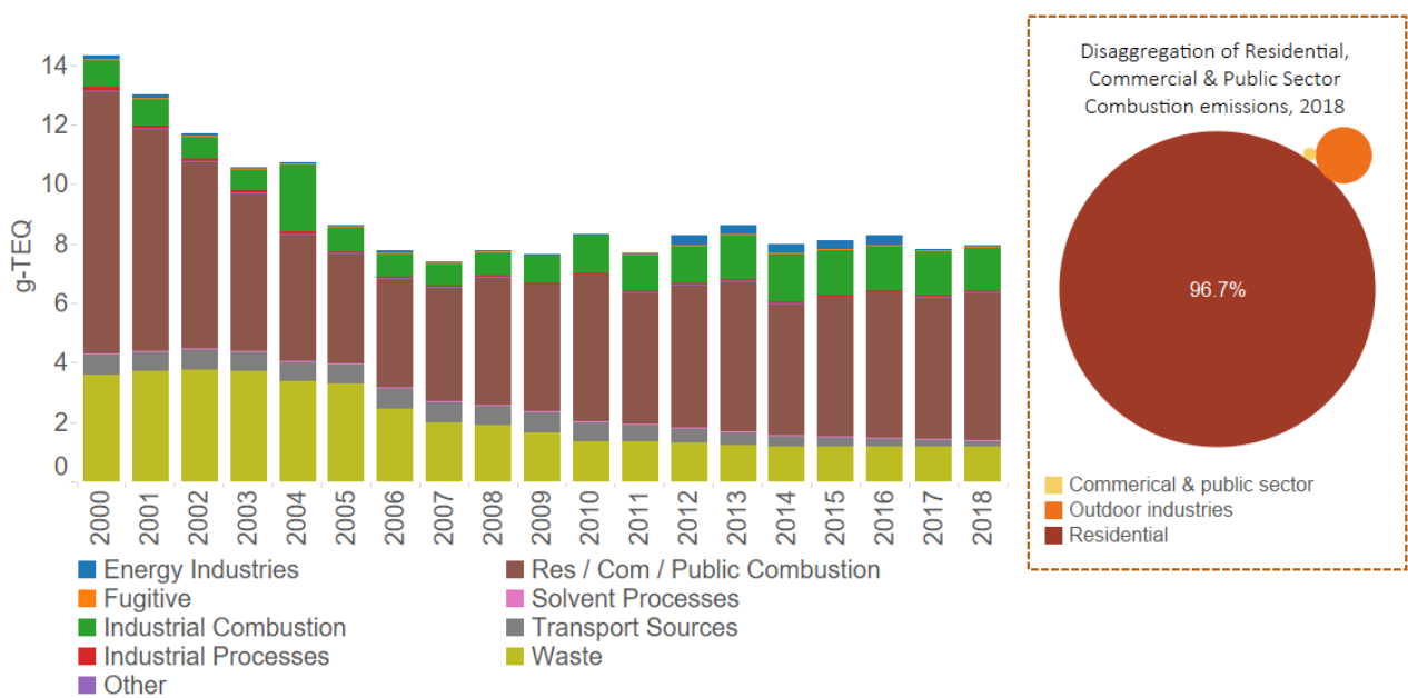
Figure 81 Dioxins Emissions in Northern Ireland
