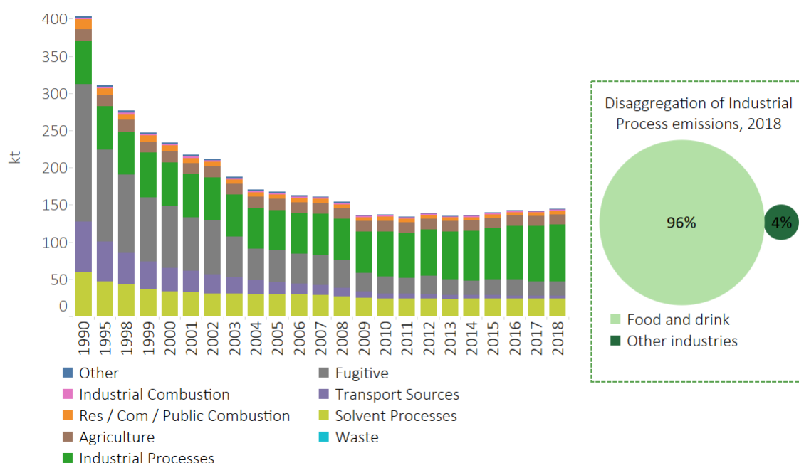
Figure 22 – NMVOC Emissions in Scotland
