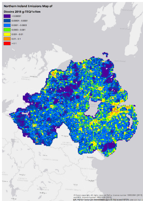
Figure 83 Dioxin Emissions in Northern Ireland, 2018
