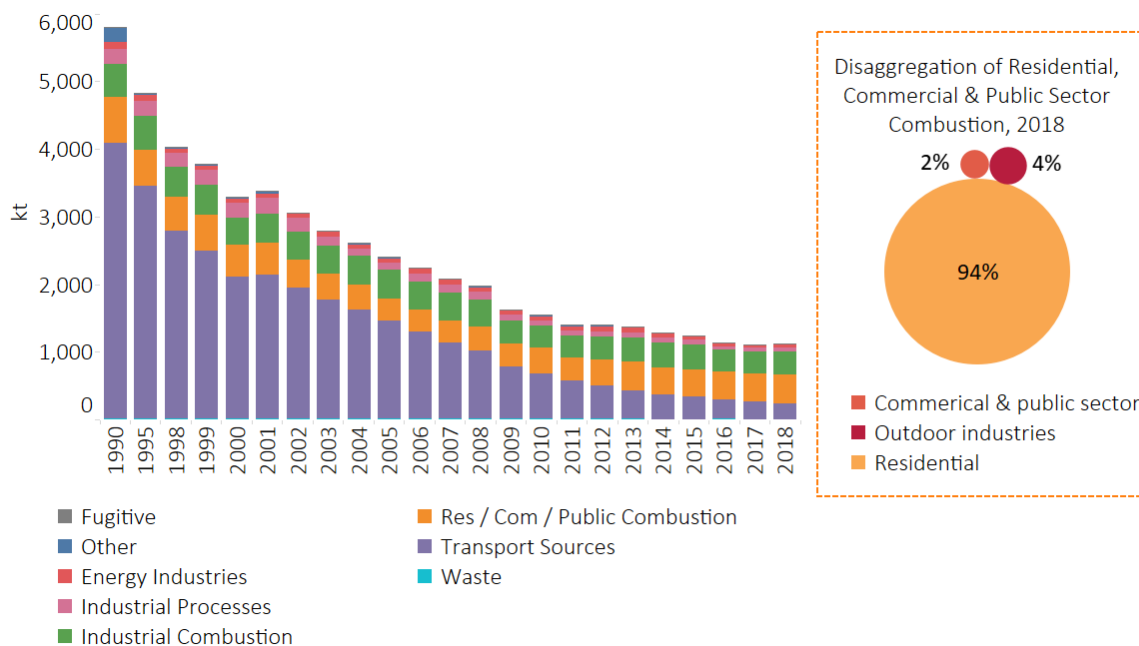
Figure 3 – Carbon Monoxide Emissions in England
