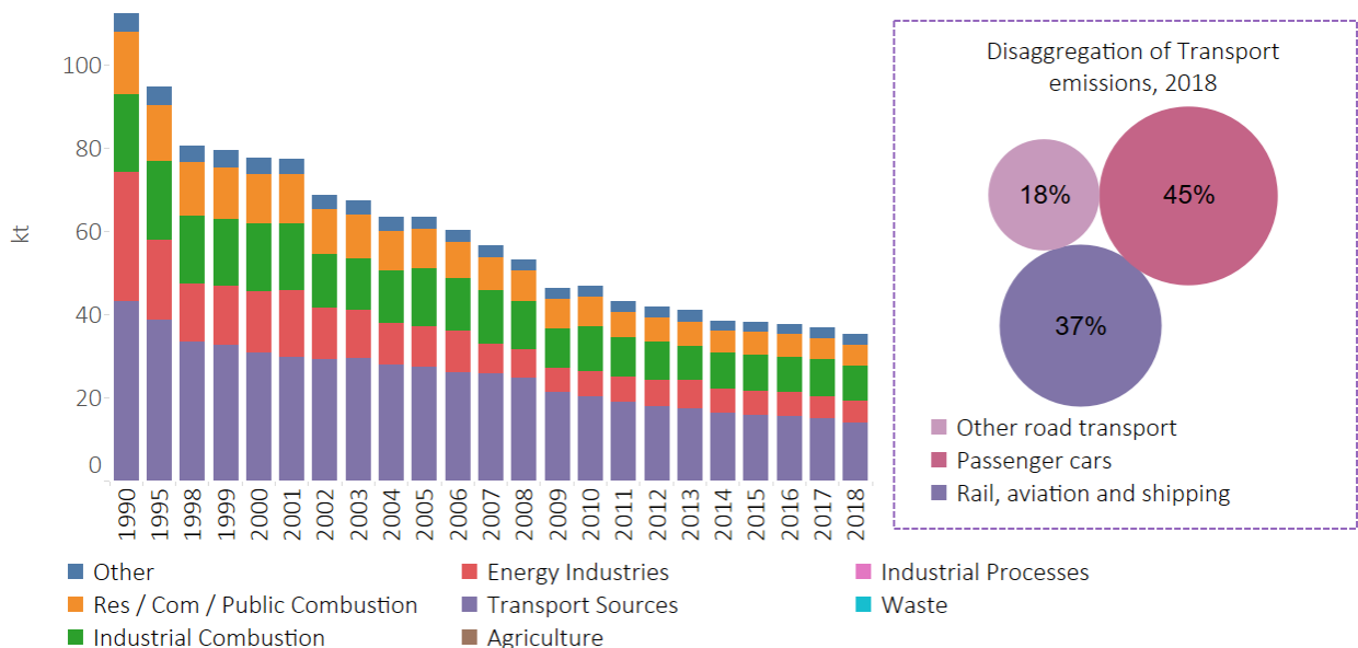
Figure 55 - Nitrogen Oxides Emissions in Northern Ireland
