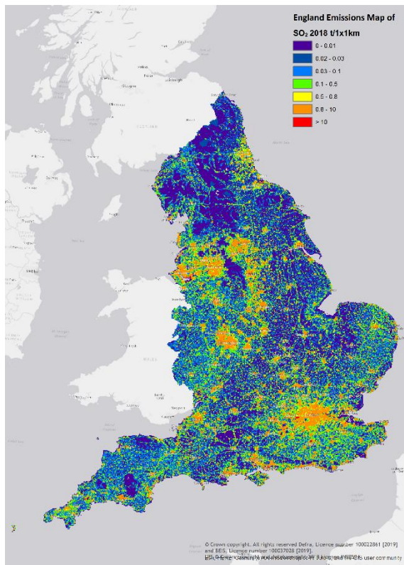
Figure 17 – Sulphur Dioxide Emissions in England, 2018
