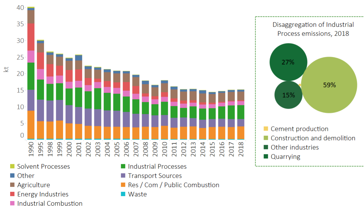
Figure 23 – PM 10 Emissions in Scotland 2
