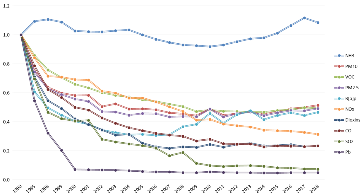
Figure 52 – Northern Ireland normalised trends for all pollutants
