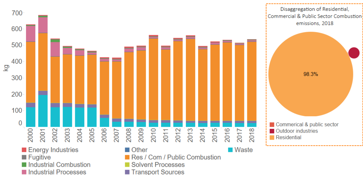
Figure 74 – B[a]p emissions in Scotland
