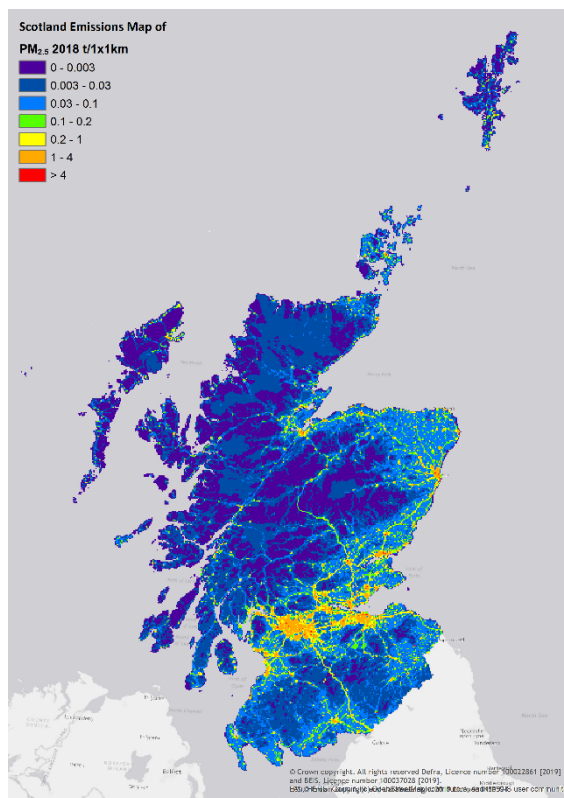
Figure 32 – PM 2.5 Emissions in Scotland, 2018
