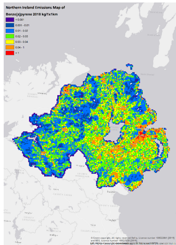
Figure 84 B[a]p Emissions in Northern Ireland, 2018
