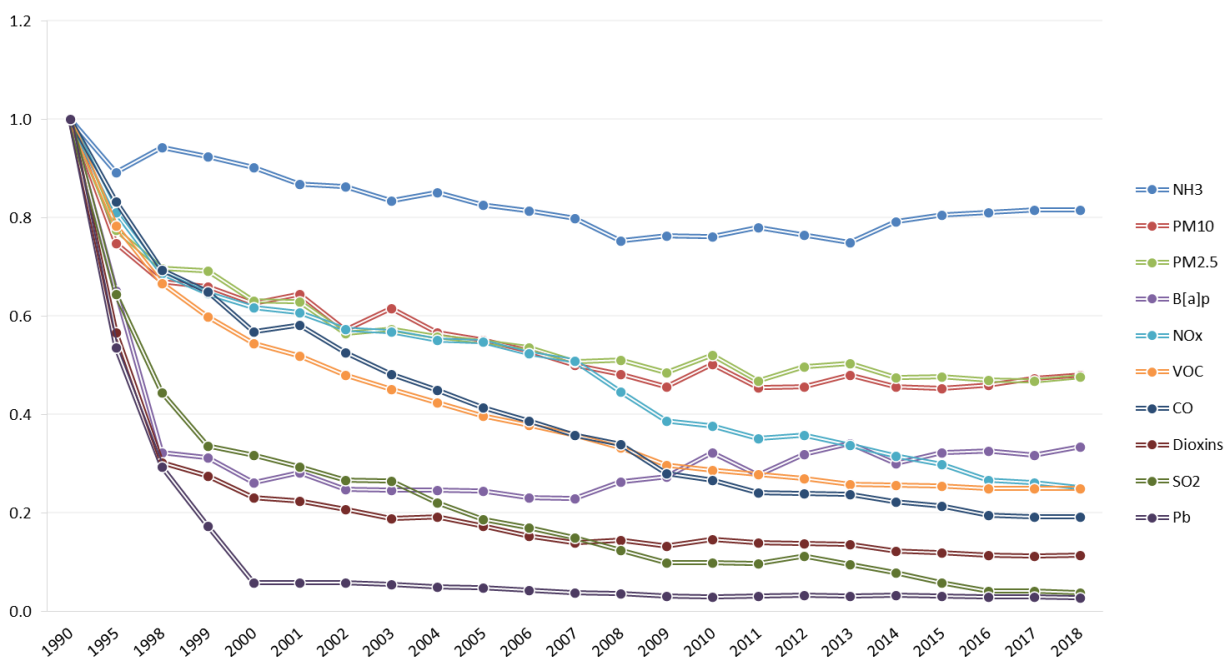
Figure 1 – England normalised trends for all pollutants
