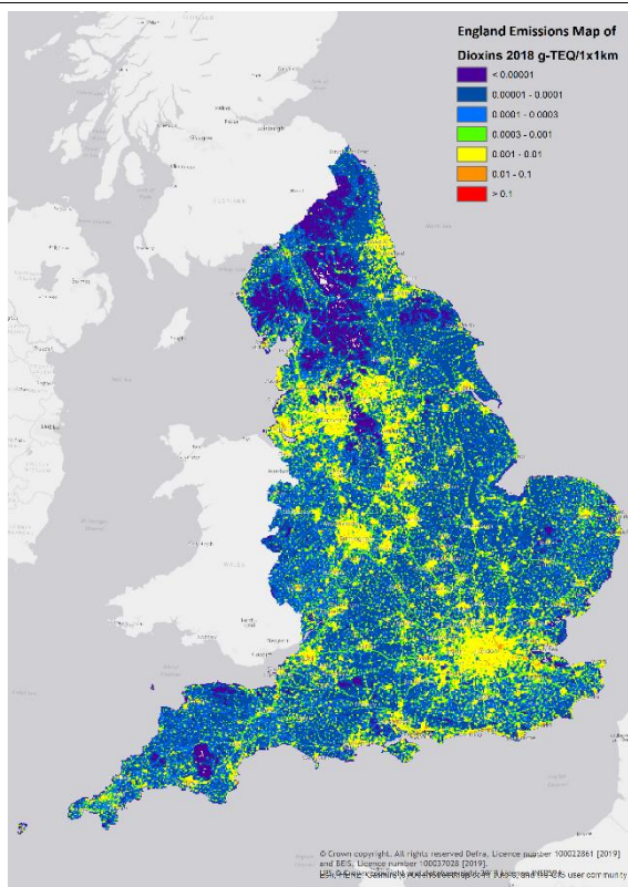
Figure 71 Dioxin Emissions in England, 2018
