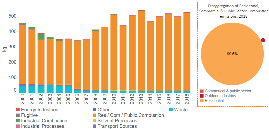
Figure 82 B[a]p Emissions in Northern Ireland
