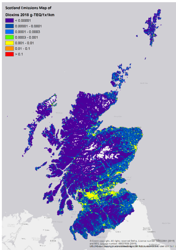
Figure 75 Dioxin Emissions in Scotland, 2018
