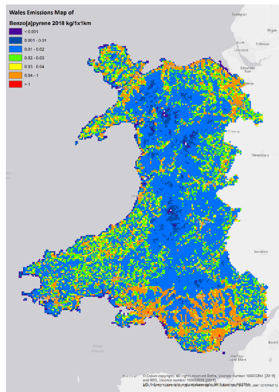
Figure 80 B[a]p Emissions in Wales, 2018
