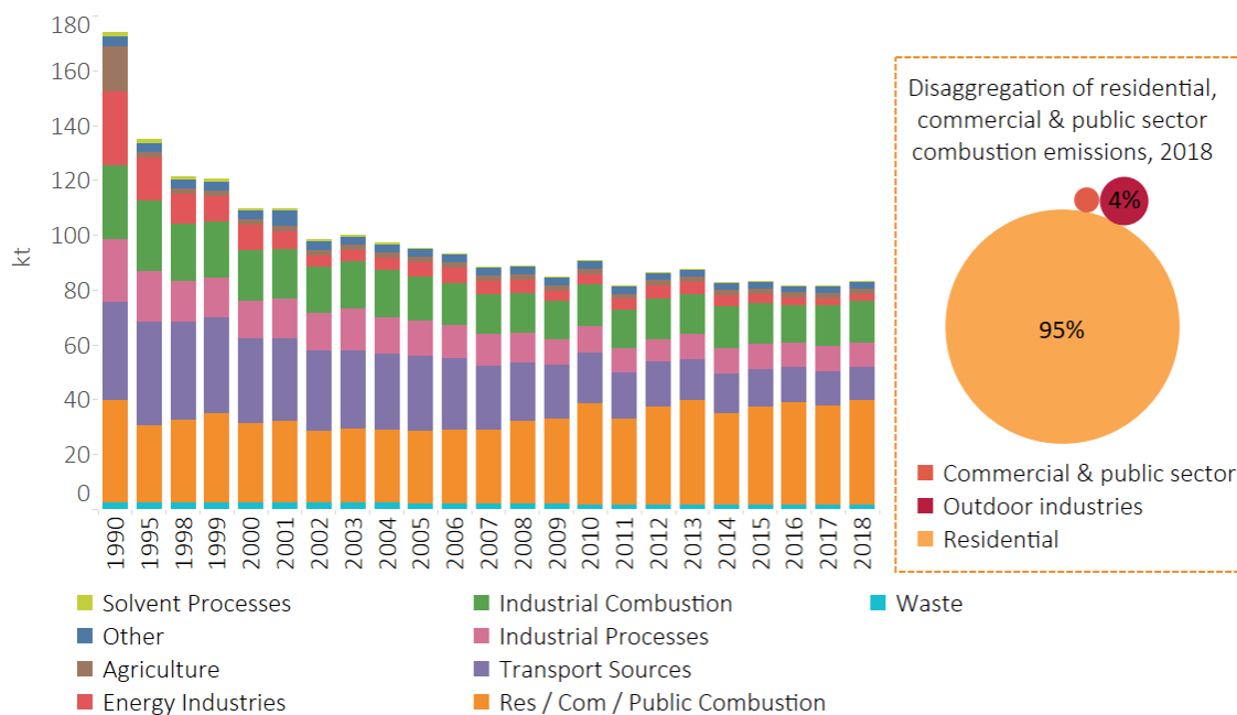
Figure 7 – PM 2.5 Emissions in England
