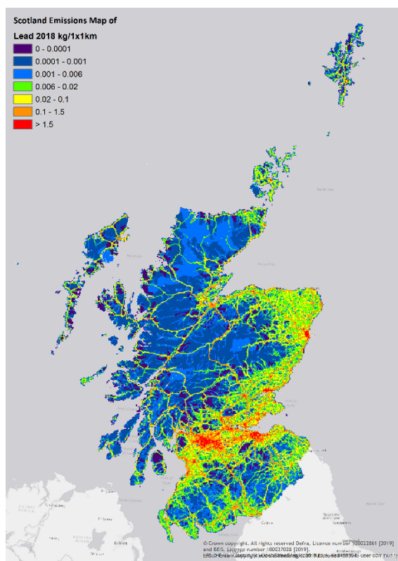
Figure 33 – Lead Emissions in Scotland, 2018
