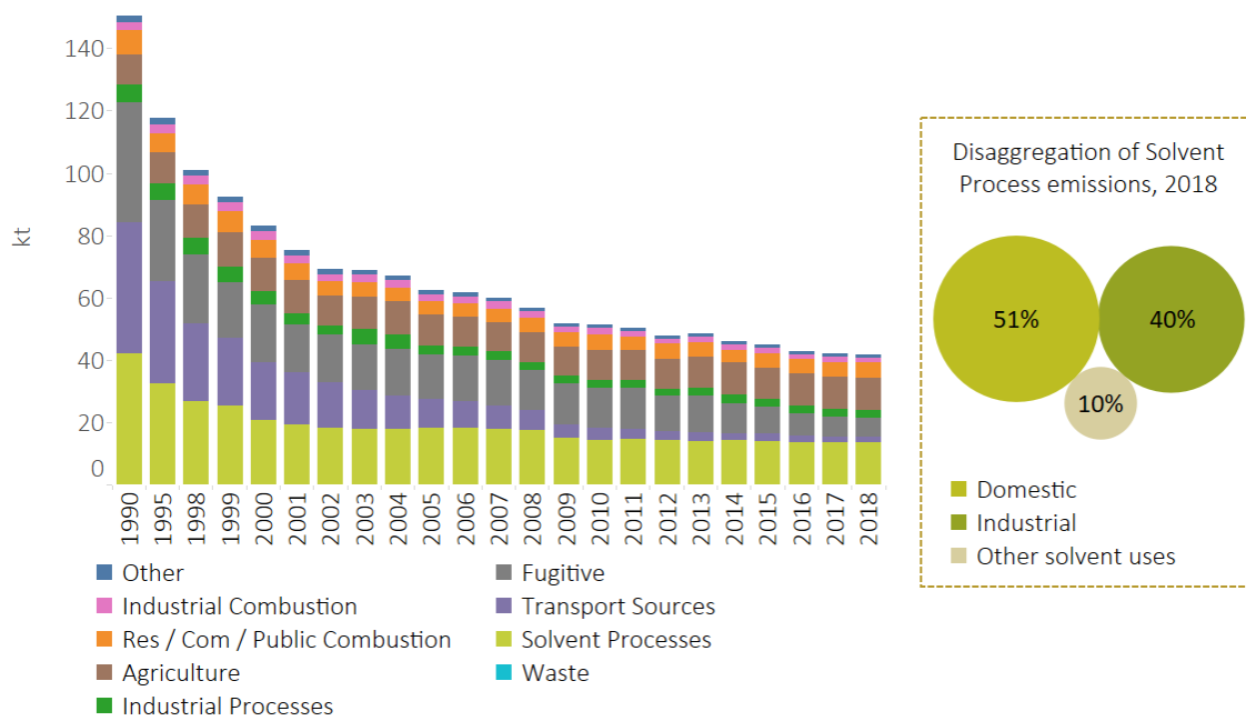
Figure 39 – NMVOC Emissions in Wales
