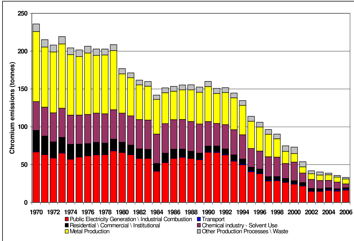
Figure 3.3 Time Series of Chromium Emissions (tonnes)
