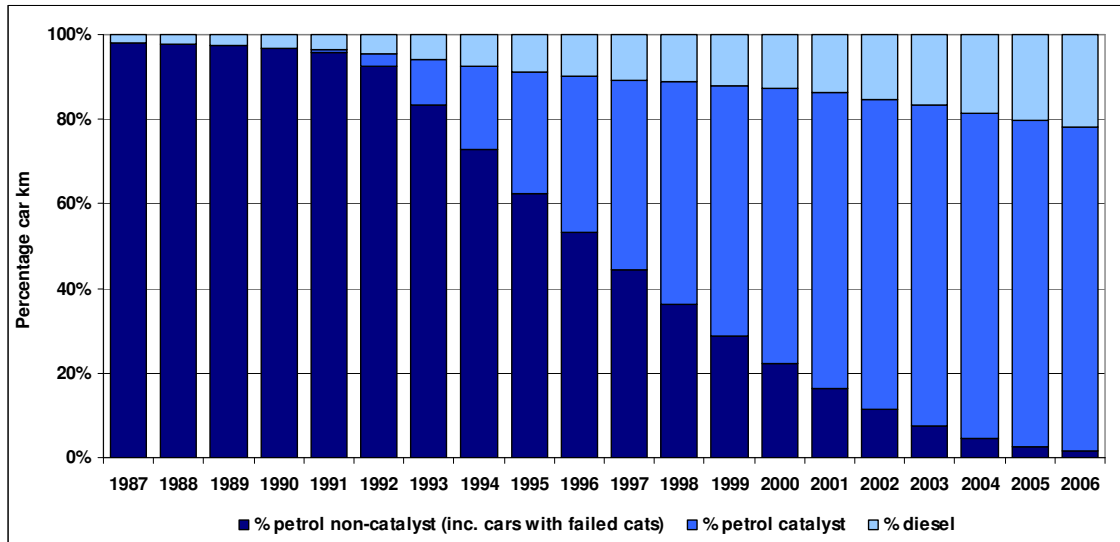
Figure 7.9 The Growth in the Number of Car Kilometres from Cars with Catalytic Converters
