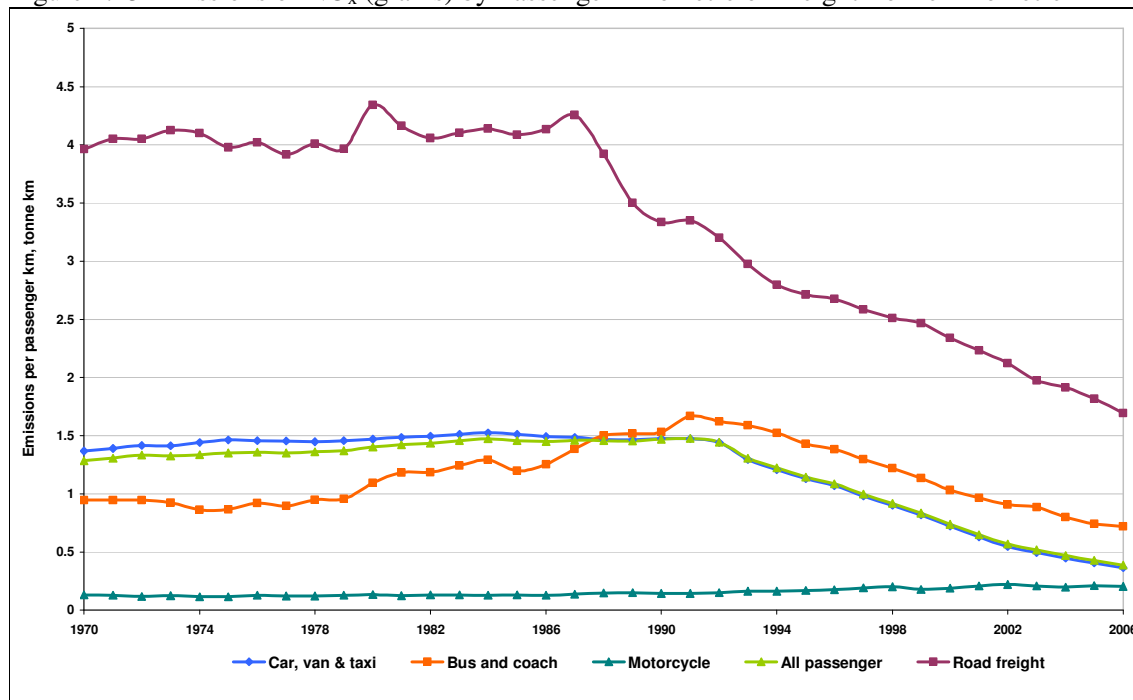
Figure 2.15 Emissions of NO x (grams) by Passenger Kilometre or Freight Tonne Kilometre
