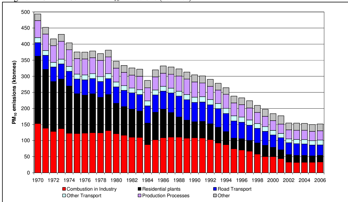
Figure 2.18 Time Series of PM 10 Emissions (ktonnes)
