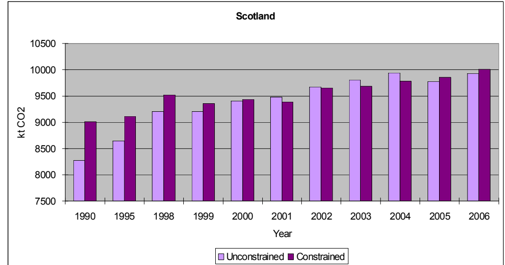
Figure A1.4.1 Road transport CO 2 emission trends 1990-2006 calculated by constrained and unconstrained methodologies
