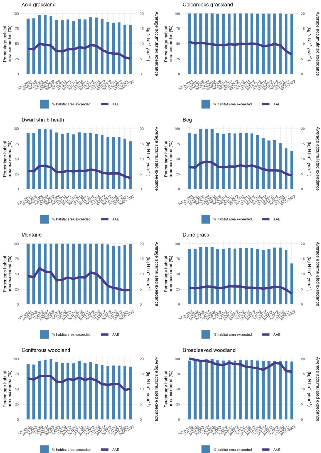
Figure 3.6: Nutrient nitrogen: Percentage area of habitats where nutrient nitrogen critical loads is exceeded, and Excess Nitrogen (AAE in kg N ha -1 year -1 ) in the UK by deposition dataset year.
