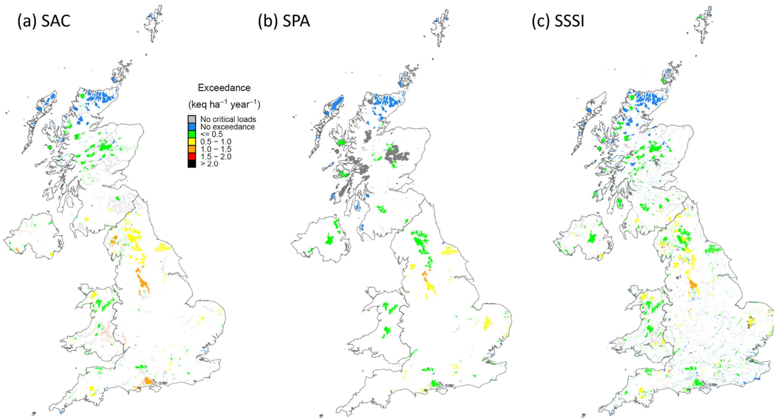
Figure 4.1: Excess Acidity. Average Accumulated Exceedance (AAE) of acidity critical loads by CBED deposition for 2019-21; maps show the maximum Excess Acidity for any feature within each site (other features may have lower or no exceedance).
