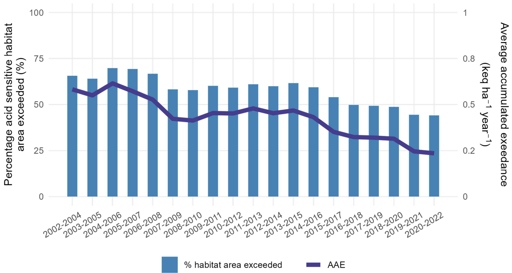
Figure 3.1: Acidity: Percentage area of acid-sensitive habitats with exceedance of acidity critical loads in the UK by year, and Average Accumulated Exceedance in keq ha -1 year -1 .
