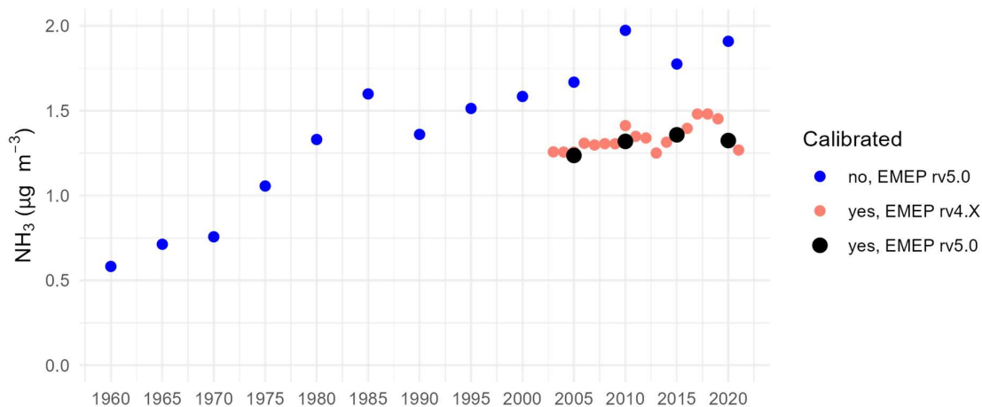
Figure 2.3 Changes in UK mean ammonia concentration since 1960 or since 2003, estimated using three approaches: release version 5.0 of the EMEP4UK model, with no calibration to observations; the same model outputs calibrated to UK EAP ammonia observations (used for UKSCAPE simulations); and release version 4.X (4.36-4.45) of the EMEP4UK model with calibration to UK EAP ammonia observations (used for the current report).
