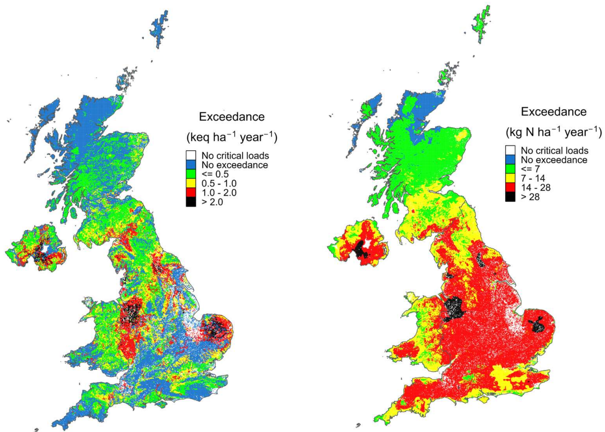
Figure 1.6: a) Excess Acidity (Average Accumulated Exceedance of acidity critical load) and b) Excess Nitrogen (Average Accumulated Exceedance of nutrient-nitrogen critical load) in 2021. Although the legends for the two maps are given in different units, the class intervals are the same (e.g. 7 \text{ kg N ha}^{-1} \text{ year}^{-1} is equal to 0.5 \text{ keq ha}^{-1} \text{ year}^{-1} ).
