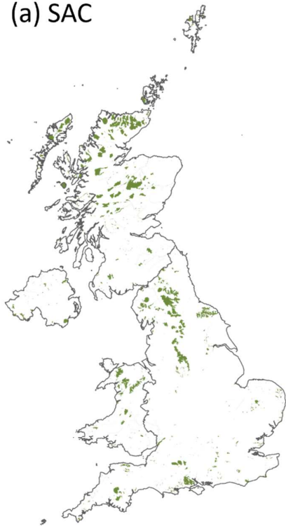
Figure 1.1: Distribution of terrestrial SACs, SPAs and SSSIs / ASSIs in the UK.
