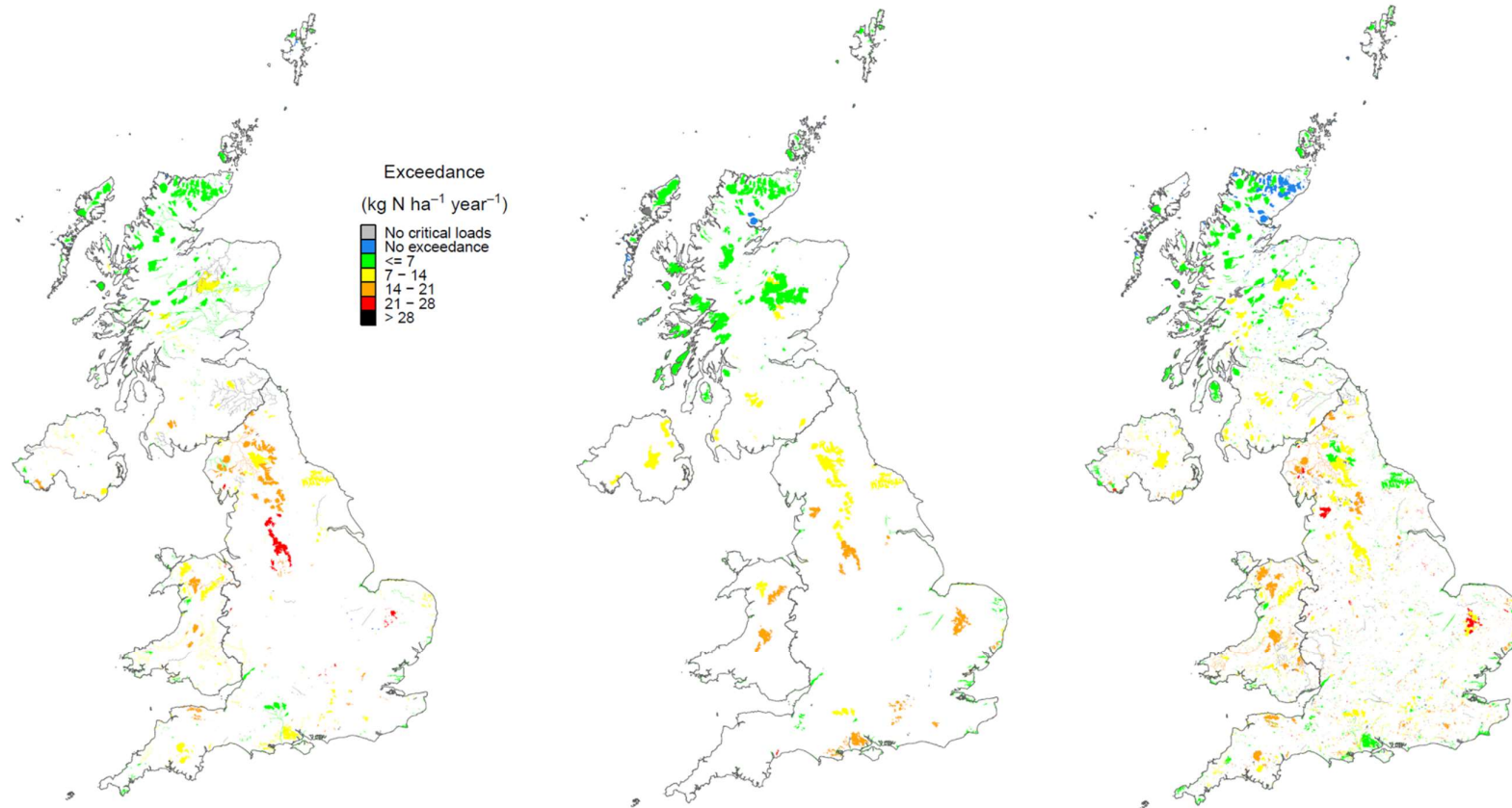
Figure 4.2: Excess Nitrogen: Average Accumulated Exceedance (AAE) of nutrient nitrogen critical loads by CBED deposition for 2019-21. Maps show the maximum AAE for any feature within each site. Other features may have lower or no exceedance. Note that small sites may not show at this resolution.
