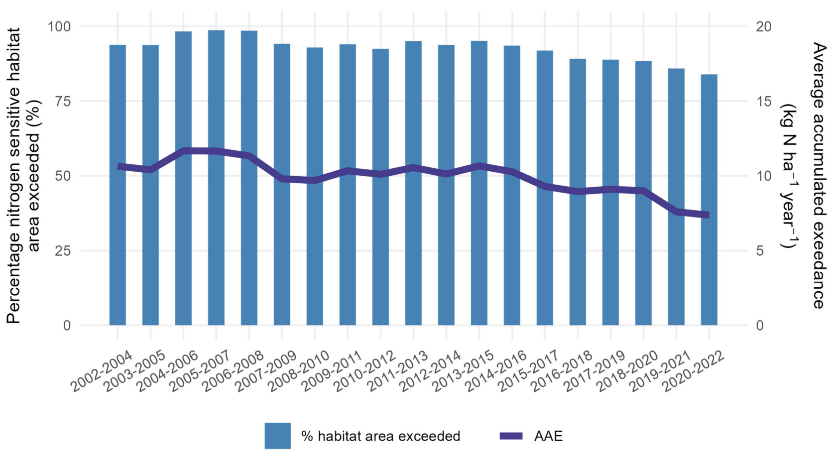
Figure 3.3: Nutrient nitrogen: Percentage area of nitrogen-sensitive habitats with exceedance of nitrogen critical loads in the UK by year, and Excess Nitrogen (Average Accumulated Exceedance in kg N ha -1 year -1 ).
