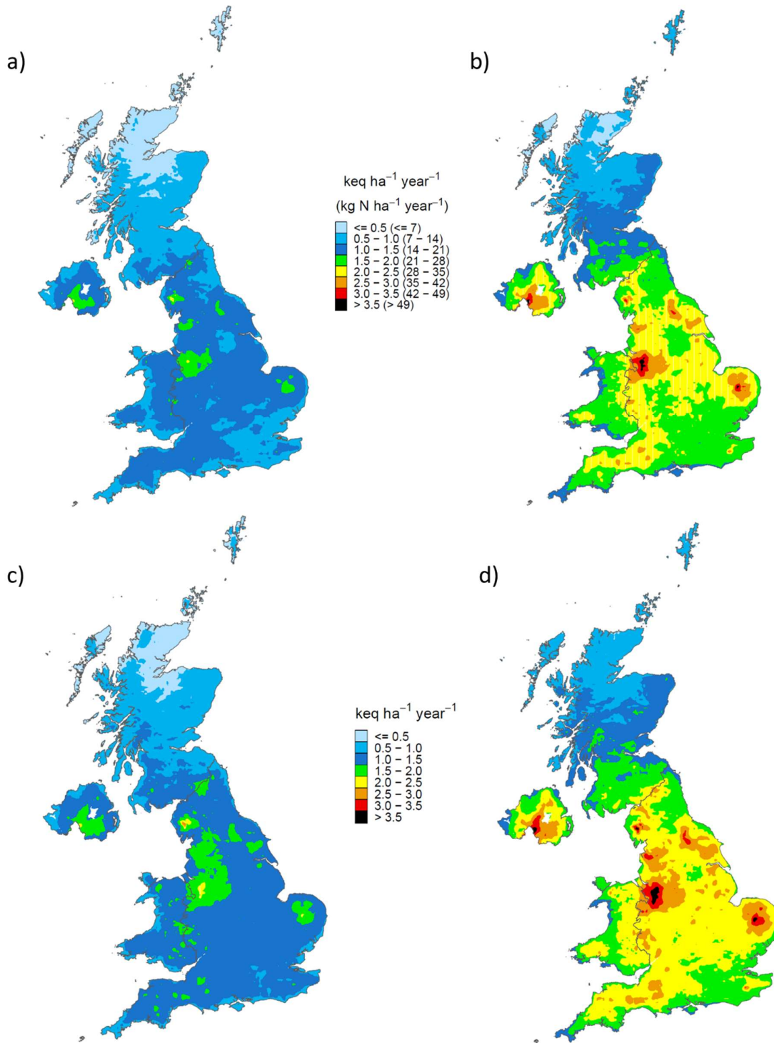
Figure 1.2: CBED deposition for 2020-2022: a) nitrogen (oxidised plus reduced) deposition to moorland; b) nitrogen (oxidised plus reduced) deposition to woodland; c) acid (sulphur + nitrogen) deposition to moorland; d) acid (sulphur + nitrogen) deposition to woodland. Deposition is mapped for N and acidity using the same units ( \text{keq ha}^{-1} \text{ yr}^{-1} ) and class intervals. For the N maps, deposition rates are also shown in \text{kg N ha}^{-1} \text{ yr}^{-1} .
