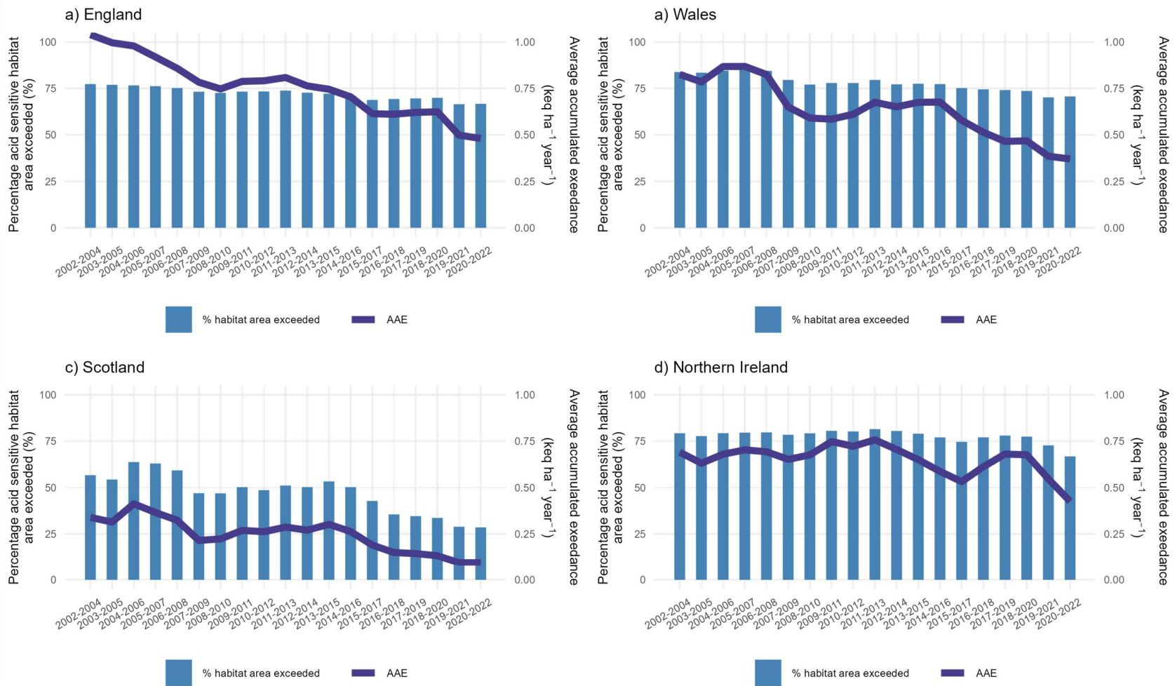
Figure 3.2: Acidity: Percentage area of acid-sensitive habitats with exceedance of acidity critical loads, by country and year, and Excess Acidity (Average Accumulated Exceedance in \text{keq ha}^{-1} \text{ year}^{-1} ).
