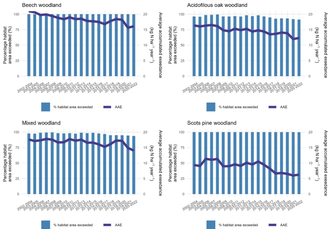
Figure 3.6 (continued): Nutrient nitrogen: Percentage area of habitats where nutrient nitrogen critical load is exceeded, and Excess Nitrogen (Average Accumulated Exceedance in kg N ha -1 year -1 ) in the UK by deposition dataset year.
