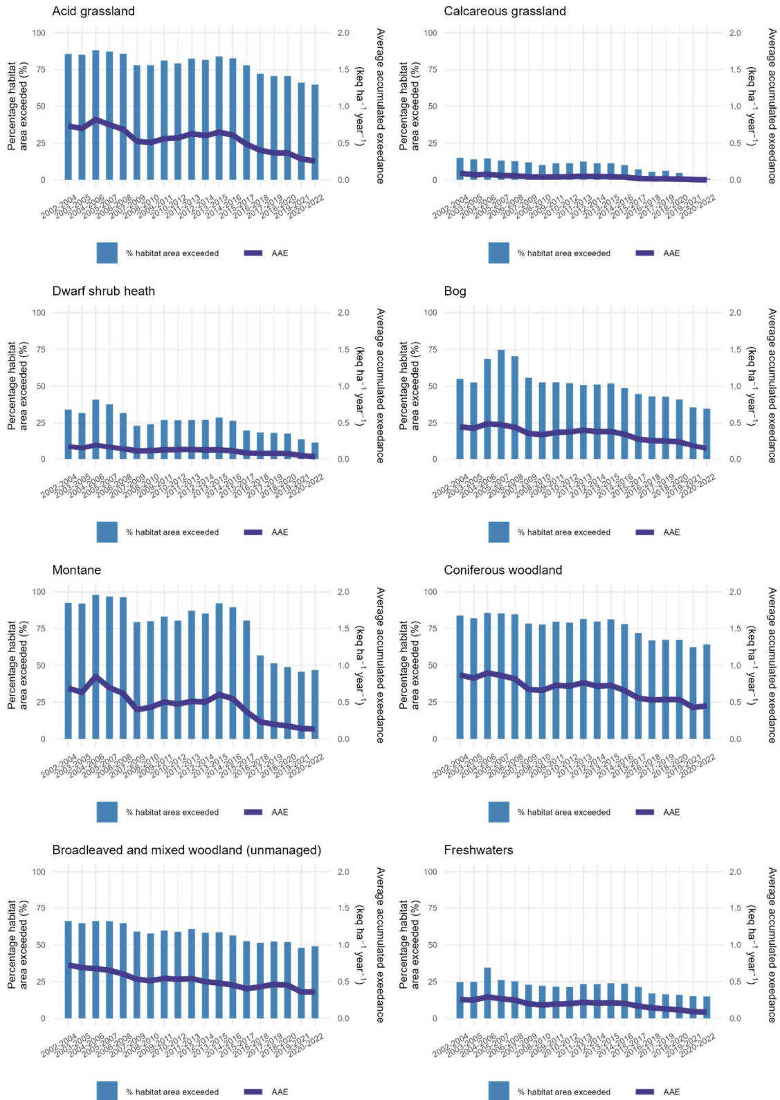
Figure 3.5: Acidity: Percentage area of habitats where acidity critical loads are exceeded, and Excess Acidity (AAE in keq ha -1 year -1 ) for the UK by deposition dataset year.
