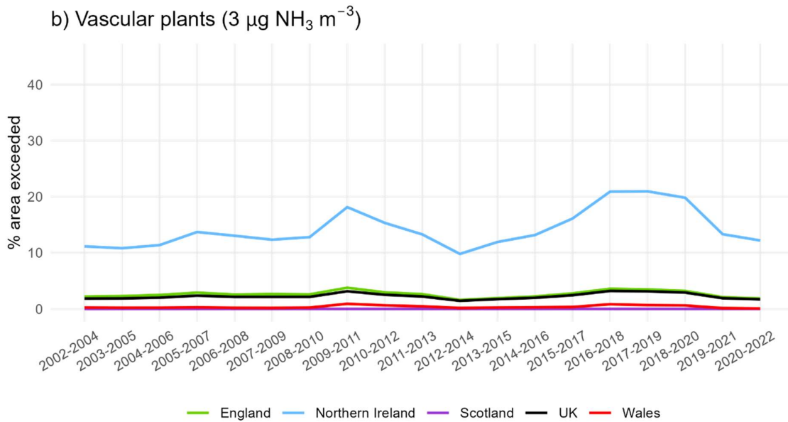
Figure 2.1: Percentages of the UK land area where ammonia concentrations exceeded critical levels: for a) lichens and bryophytes; b) vascular plants.
