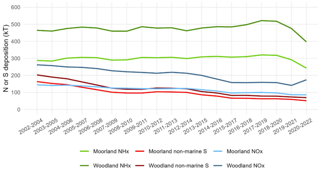
Figure 1.3: Deposition budgets (kilotonnes S or N per year) calculated by CBED using ammonia concentration maps from EMEP assuming UK area is a) woodland or b) moorland or other unfertilised open habitat. NMS = non-marine sulphur, NOx = oxidised nitrogen, NHx = reduced nitrogen.
