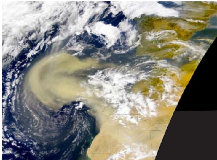
Figure 4.24: Saharan Dust Plume, from SeaWifs
