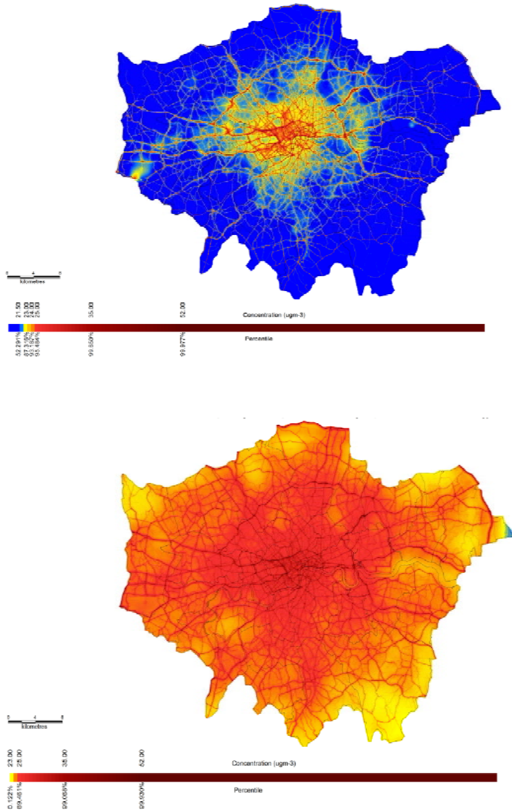
Figure 4.14: Modelled 2005 Annual Mean PM 10 concentration ( \mu\text{g m}^{-3} ) in London based on 2002 (top) and 2003 (bottom) meteorological data (Greater London Authority, personal communication)
