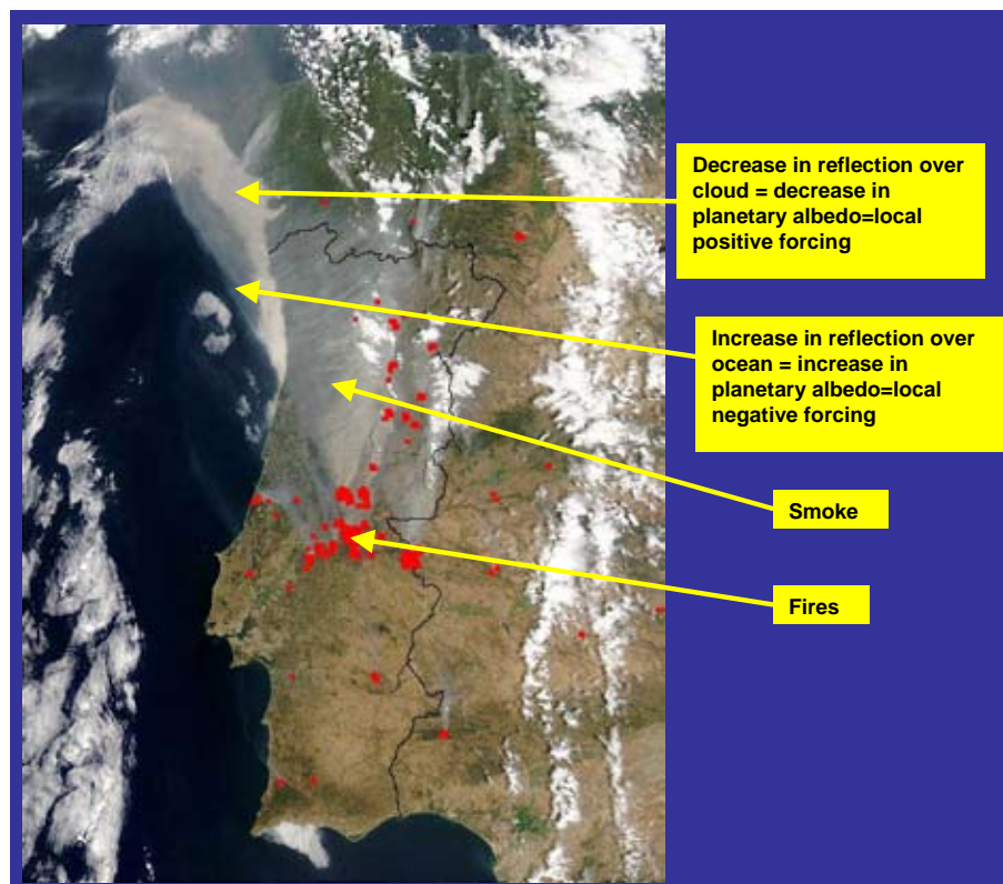
Figure 3.9: MODIS image showing the emission of biomass smoke from Portugal on 3 August 2003
