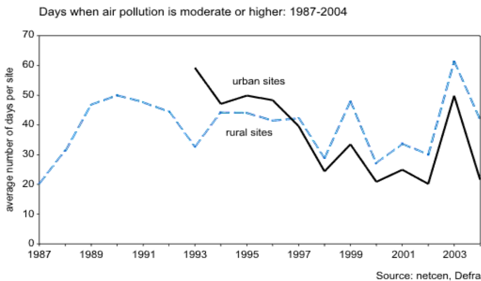
Figure 4.13: UK Headline Air Quality Indicator 1987 – 2004
