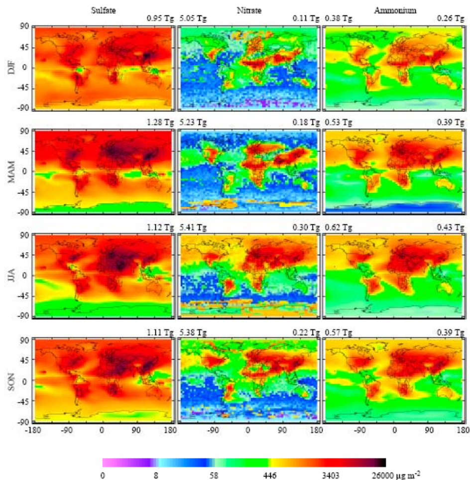
Figure 3.10: Seasonal mass column concentrations of aqueous sulphate, nitrate, and ammonium calculated by Martin et al. (2004)
