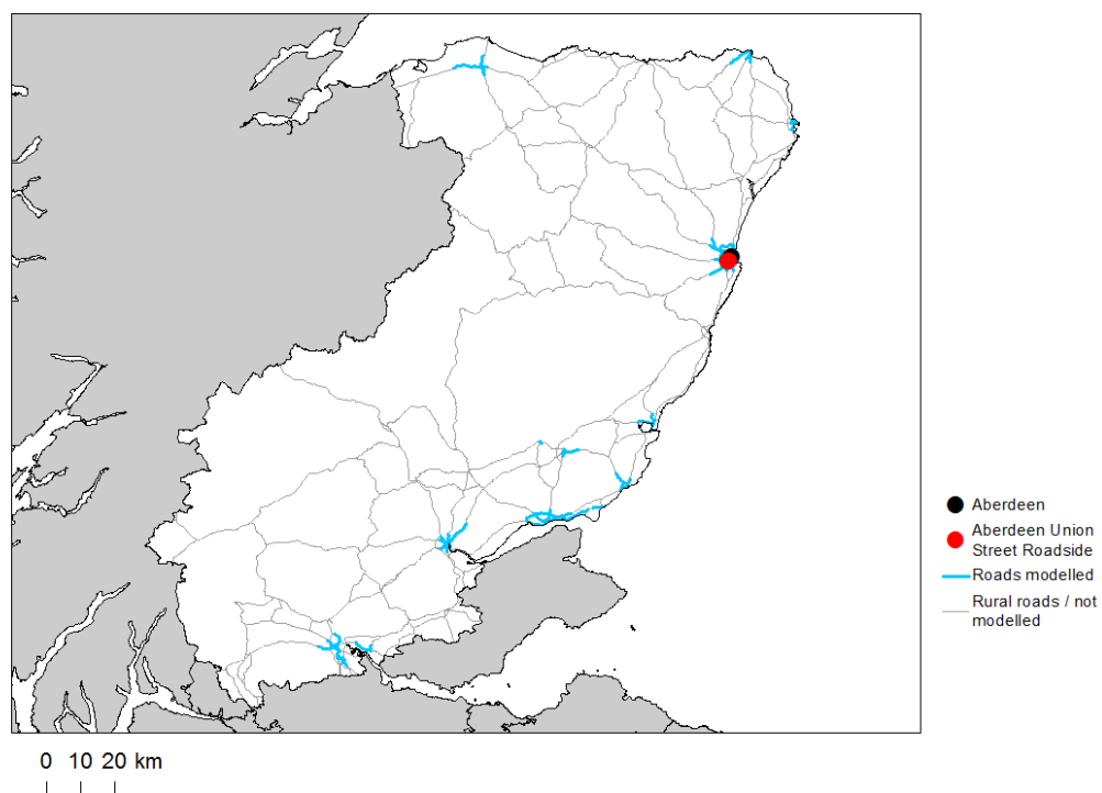
Figure 3: Map showing the location of the NO 2 monitoring stations with valid data in 2013 and roads where concentrations have been modelled within the North East Scotland (UK0038) non-agglomeration zone.
