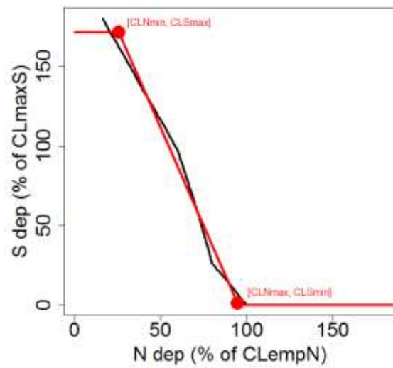
Figure 6.3: Response of habitat quality of an acid grassland Special Area for Conservation, Hill of Towanreef, to nitrogen (N) and sulphur (S) deposition scenarios: a) response illustrated in a '3D' plot; b) combinations of N and S deposition resulting in a critical value for habitat quality, HQI_{crit} ; c) simplified version of the HQI_{crit} response function.
