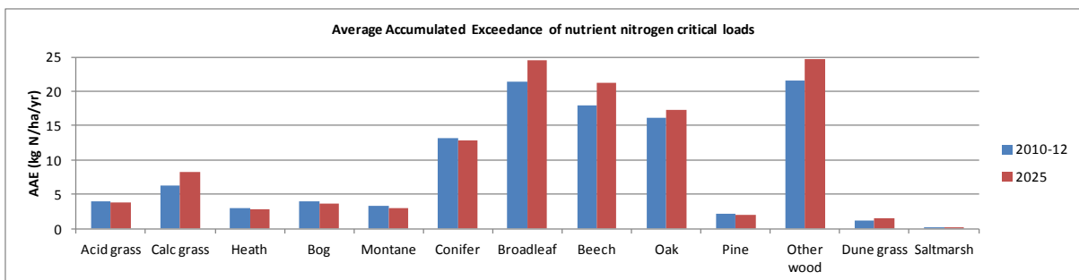
Figure 8.3: AAE for nutrient nitrogen by habitat for the UK, comparing results based on CBED 2010-12 and FRAME 2025 (UEP45) deposition.
