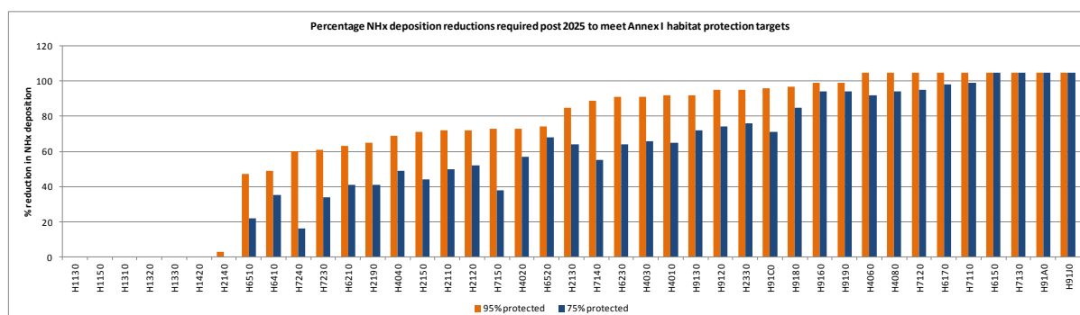
Figure 10.1: Plot showing the percentage reductions in NHx deposition required to meet the 75% and 95% protection targets for 41 Annex I habitats. Bars plotted above 100% represent those habitats where targets can only be met if all NHx deposition is removed AND reductions are also made in NOx deposition.
