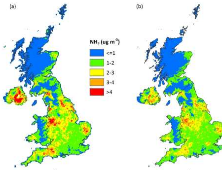
Figure 2.7: Mean NH 3 concentrations for 2010-12 at (a) 5km resolution from CBED, and (b) 1km resolution from FRAME.
