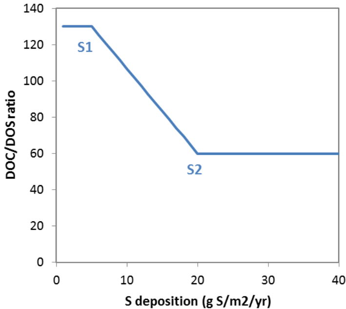
Figure 9.2: Response function for the relationship between peat porewater DOC/DOS ratio and total (marine plus non-marine) S deposition, based on peat core data (Section 9.2). Point S1 represents the S deposition at which the peat S accumulation begins to rise above background rates, and point S2 represents the S deposition at which the maximum rate of peat S accumulation occurs.
