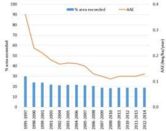
Figure 3.3 (g-h): Acidity: UK results of the percentage area of acid-sensitive habitats* with exceedance of critical loads and the Average Accumulated Exceedance (keq ha -1 year -1 ). For information on the CBED deposition data used refer to Section 2.1. * "Freshwaters" results were based on data for 1752 freshwater catchments in the UK. For further information please refer to Hall et al, 2015a.
