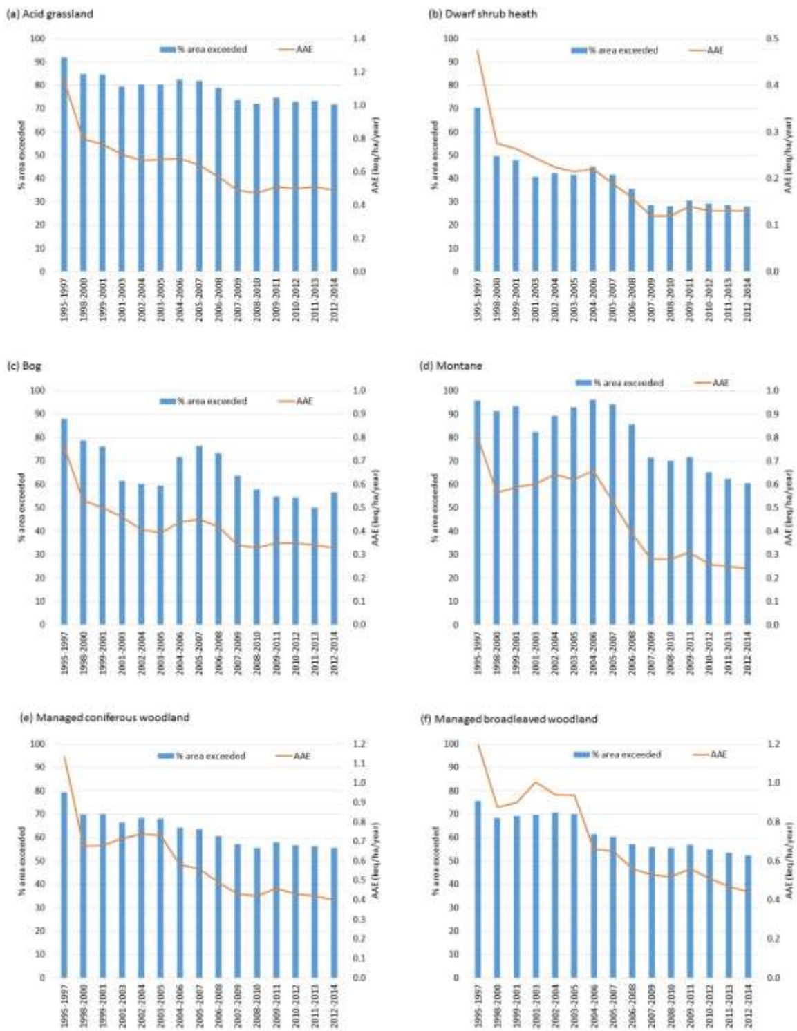
Figure 3.3 (a-f): Acidity: UK results of the percentage area of acid-sensitive habitats* with exceedance of critical loads and the Average Accumulated Exceedance ( \text{keq ha}^{-1} \text{ year}^{-1} ). For information on the CBED deposition data used refer to Section 2.1. * “Freshwaters” results were based on data for 1752 freshwater catchments in the UK. For further information please refer to Hall et al, 2015a.
