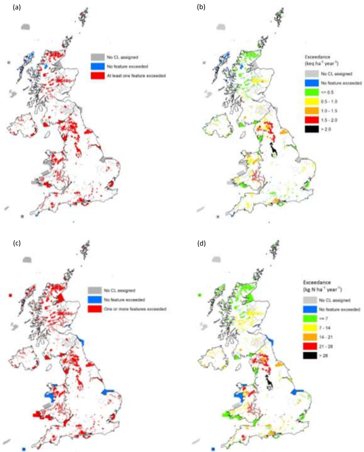
Figure 3.8: Critical load exceedance maps for SACs: (a) sites with exceedance of acidity critical loads for one or more features; (b) maximum Average Accumulated Exceedance (AAE) per site for acidity; (c) sites with exceedance of nutrient nitrogen critical loads for one or more features; (d) maximum Average Accumulated Exceedance (AAE) per site for nutrient nitrogen. All results based on site-relevant critical loads and CBED deposition for 2012-14.
