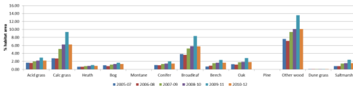
Figure 3.10: Percentage habitat area where NH 3 concentrations exceed 3 µg m -3 .
