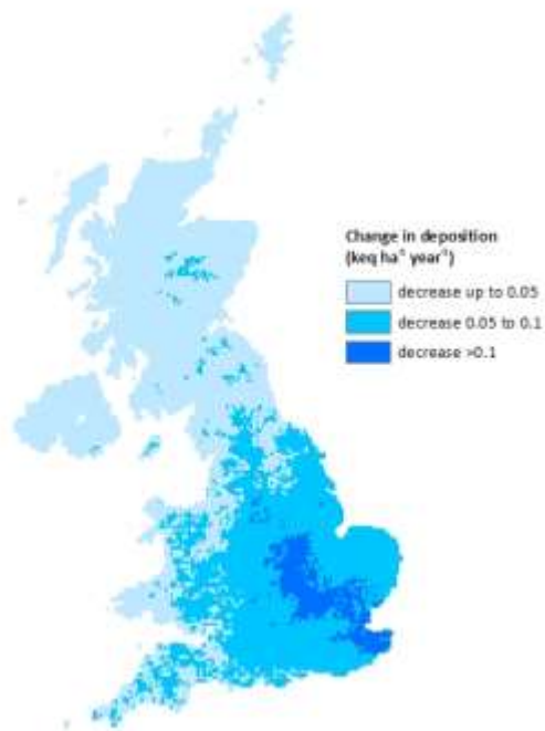
Figure 2.3: Map to show the spatial pattern of reductions in total nitrogen deposition to moorland for 2010-12, following the updates to the CBED methodology to correct for the over-estimate of nitric acid deposition. To convert from \text{keq ha}^{-1} \text{ year}^{-1} to \text{kg N ha}^{-1} \text{ year}^{-1} multiply by 14 (i.e. 0.1 \text{ keq ha}^{-1} \text{ year}^{-1} = 1.4 \text{ kg N ha}^{-1} \text{ year}^{-1} ).
