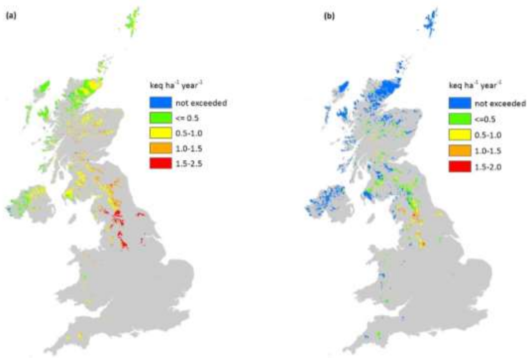
Figure 9.5: Exceedance of CLmaxS for peat soils by FRAME sulphur deposition for a hindcast scenario for 1970 for (a) critical loads based on the current methodology, and (b) the new methodology. Grey denotes areas of the UK dominated by non-peat soils.
