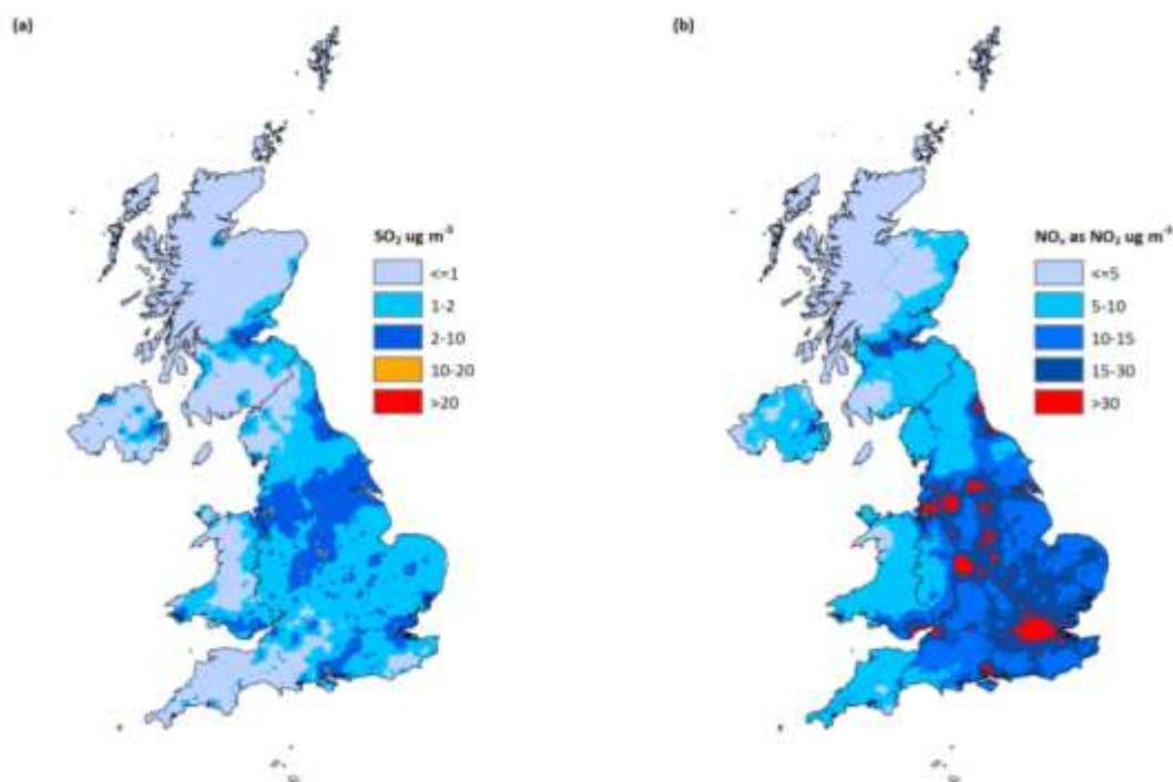
Figure 2.6: 1km concentration data for 2009 from AEAT: (a) SO 2 ; (b) NO x . Data include urban enhancement.
