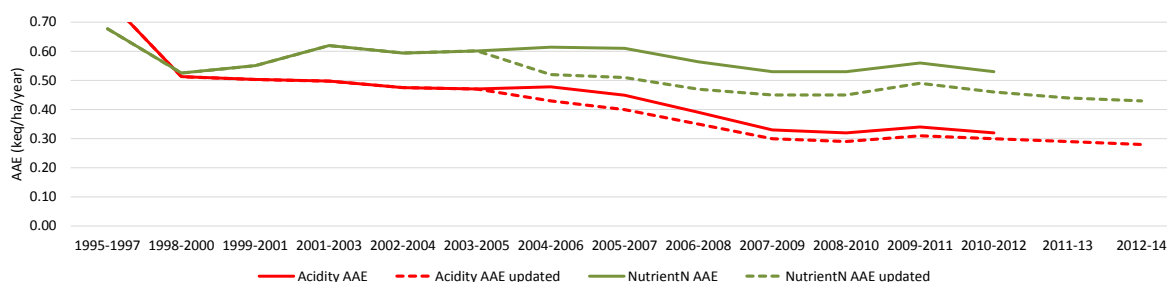
Figure 3.2: AAE of acidity and nutrient nitrogen critical loads, comparing the original results (solid line) with those based on the updated CBED deposition (dashed line).
