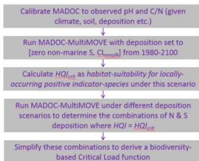
Figure 6.1: Summary of workflow used to generate biodiversity-based critical load functions using the MADOC-MultiMOVE model chain.
