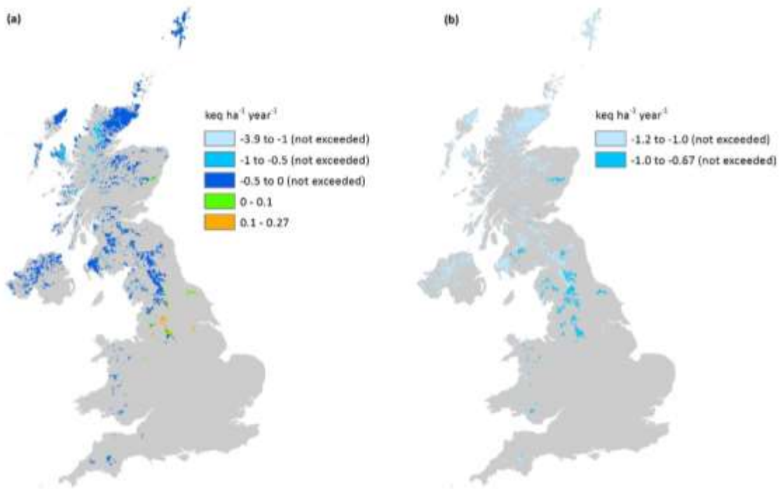
Figure 9.3: CLmaxS for peat soils in the UK based on (a) current methodology; (b) new methodology. Grey denotes areas of the UK dominated by non-peat soils.
