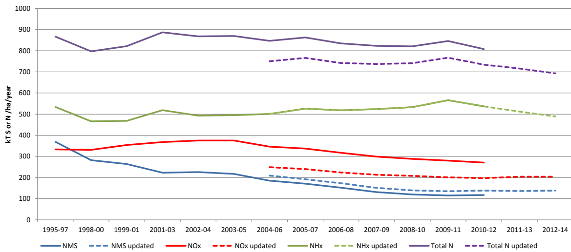
Figure 2.2: Budgets for CBED deposition to woodland; trends over time including updates to CBED 2004-2013.
