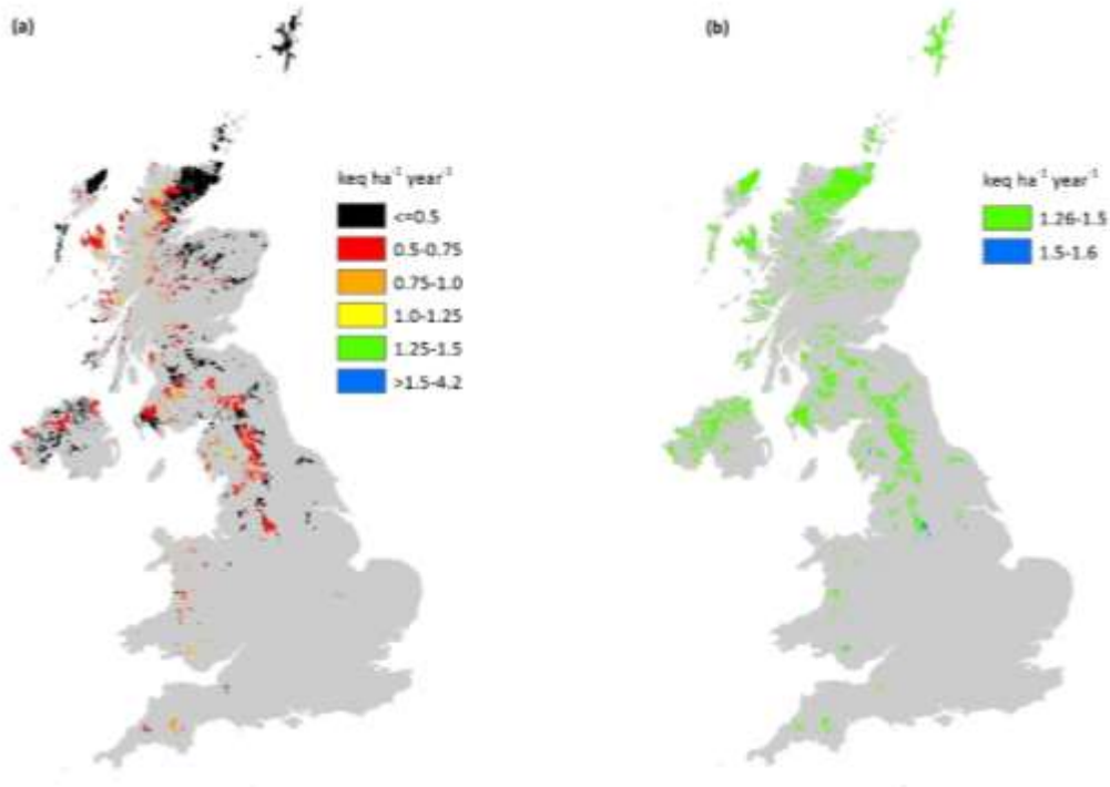
Figure 9.3: CLmaxS for peat soils in the UK based on (a) current methodology; (b) new methodology. Grey denotes areas of the UK dominated by non-peat soils.
