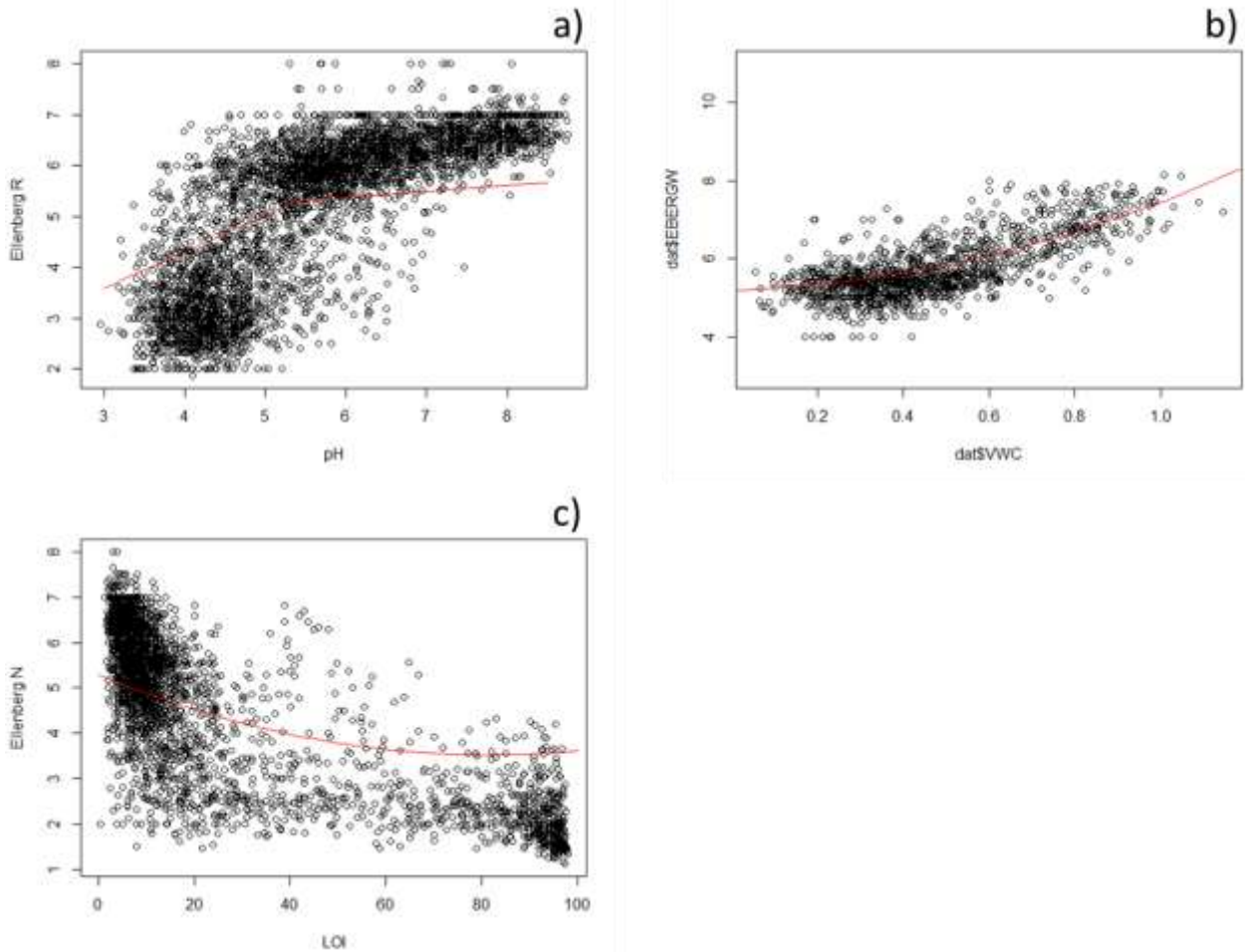
Figure 6.8: Model fits from single predictor equations for a) Ellenberg R, b) Ellenberg F, c) Ellenberg N.
