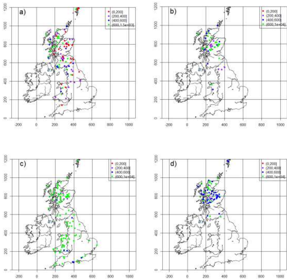
Figure 6.6. Absolute CL_{maxS} values. Special Areas of Conservation (SAC) with a) bog (EUNIS D1); b) dry acid grassland (EUNIS E1.7); c) dry heath (EUNIS F4.2); and d) wet heath (EUNIS F4.11), for which biodiversity-based Critical Load functions have been calculated. Colours indicate CL_{maxS} , expressed as eq\ ha^{-1}\ yr^{-1} i.e. as absolute values. Sites with low CL_{maxS} (red or purple) will be exceeded at low rates of S deposition compared to sites with high CL_{maxS} (blue or green).
