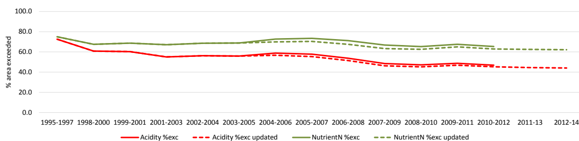
Figure 3.1: Percentage area of habitats exceeding critical loads of acidity and of nutrient nitrogen, comparing the original results (solid line) with those based on the updated CBED deposition (dashed line).
