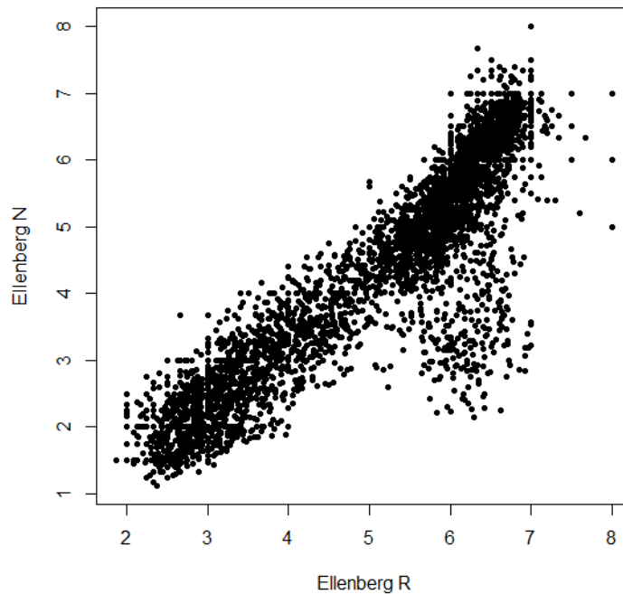
Figure 6.11: Relationship between mean Ellenberg 'R' (alkalinity) and mean Ellenberg 'N' (related to productivity or eutrophication) in the training dataset. The points with relatively high mean Ellenberg 'R' and relatively low mean Ellenberg 'N' correspond to calcareous grassland sites.
