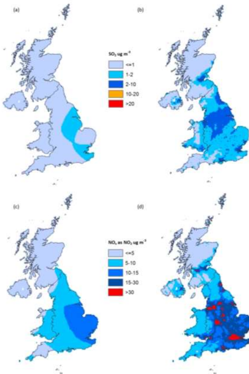
Figure 2.5: CBED 5km concentration data for 2010-12 (not updated): (a) SO 2 rural network only; (b) SO 2 rural plus urban enhancement; (c) NO x rural network only; (d) NO x rural plus urban enhancement.
