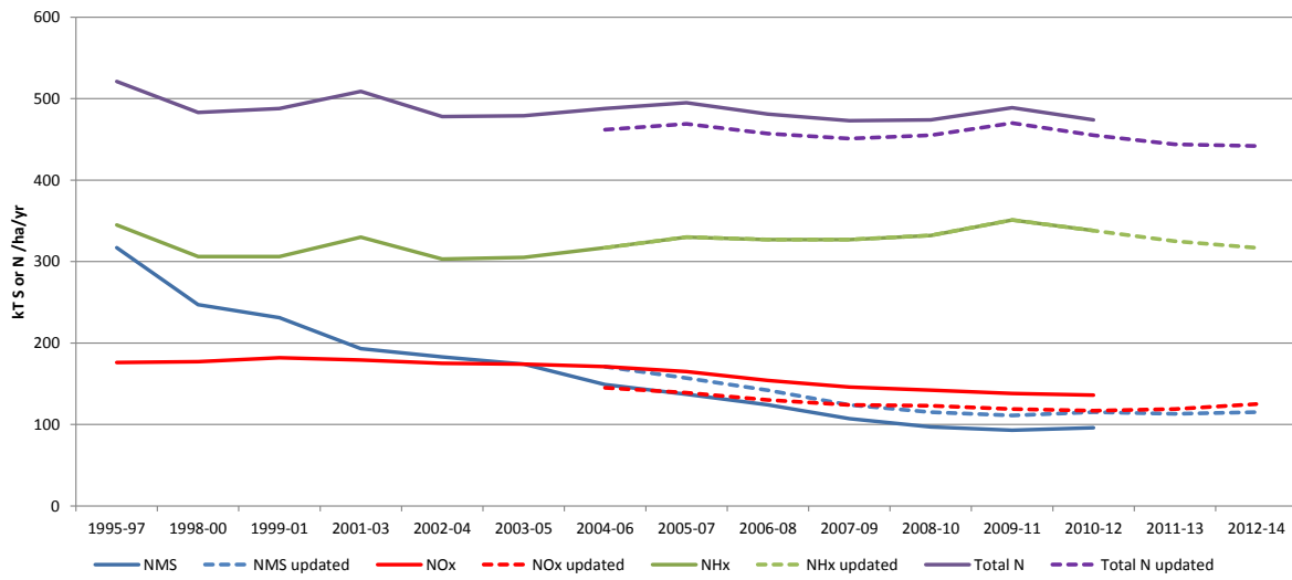
Figure 2.1: Budgets for CBED deposition to moorland; trends over time including updates to CBED 2004 to 2013.
