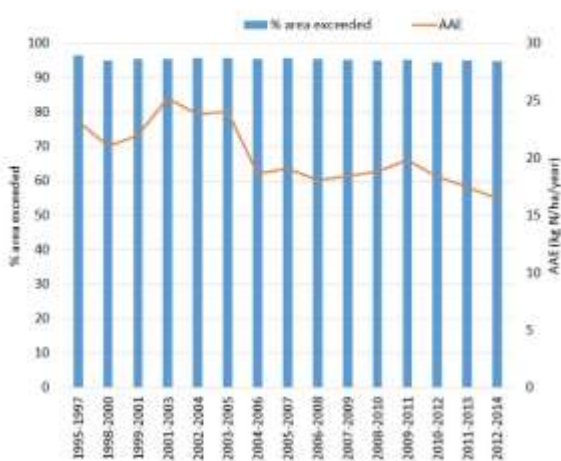
Figure 3.4 (g-l). Nutrient nitrogen: UK results of the percentage area of nitrogen-sensitive habitats* with exceedance of critical loads and the Average Accumulated Exceedance ( \text{kg N ha}^{-1} \text{ year}^{-1} ). For information on the CBED deposition data used refer to Section 2.1. * Results for Saltmarsh habitat not shown; area of habitat exceeded by CBED deposition in 1995-97 is 2% (0.7% with data for 2012-14), and the AAE is <0.1 \text{ kg N ha}^{-1} \text{ year}^{-1} in most years.
