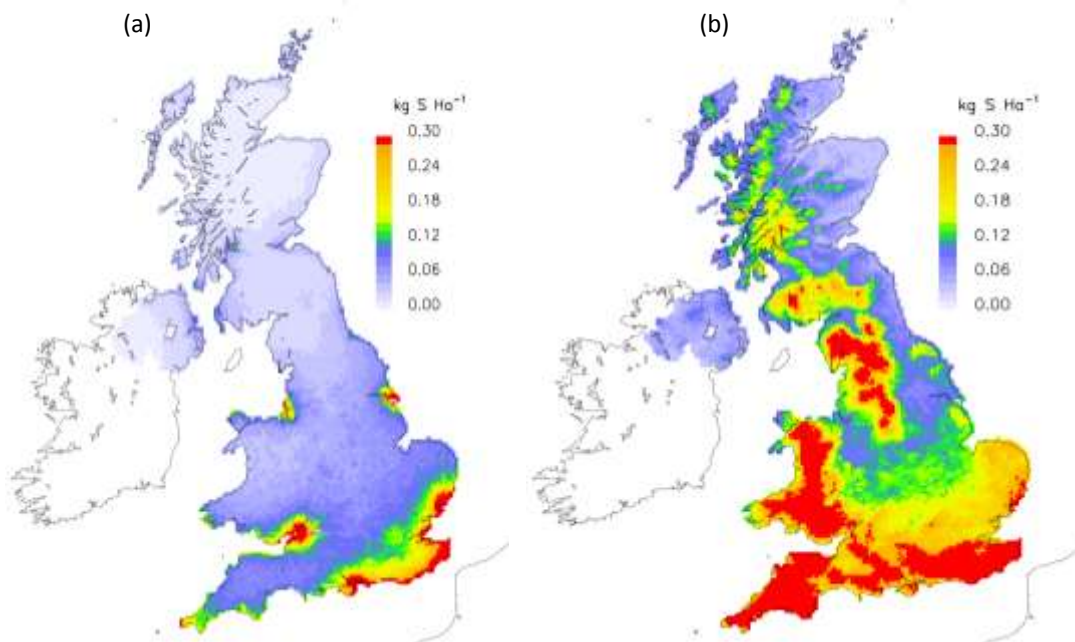
Figure 1: Reduction in: (a) dry deposition of sulphur and (b) wet deposition of sulphur between scenarios 1 and 3.
