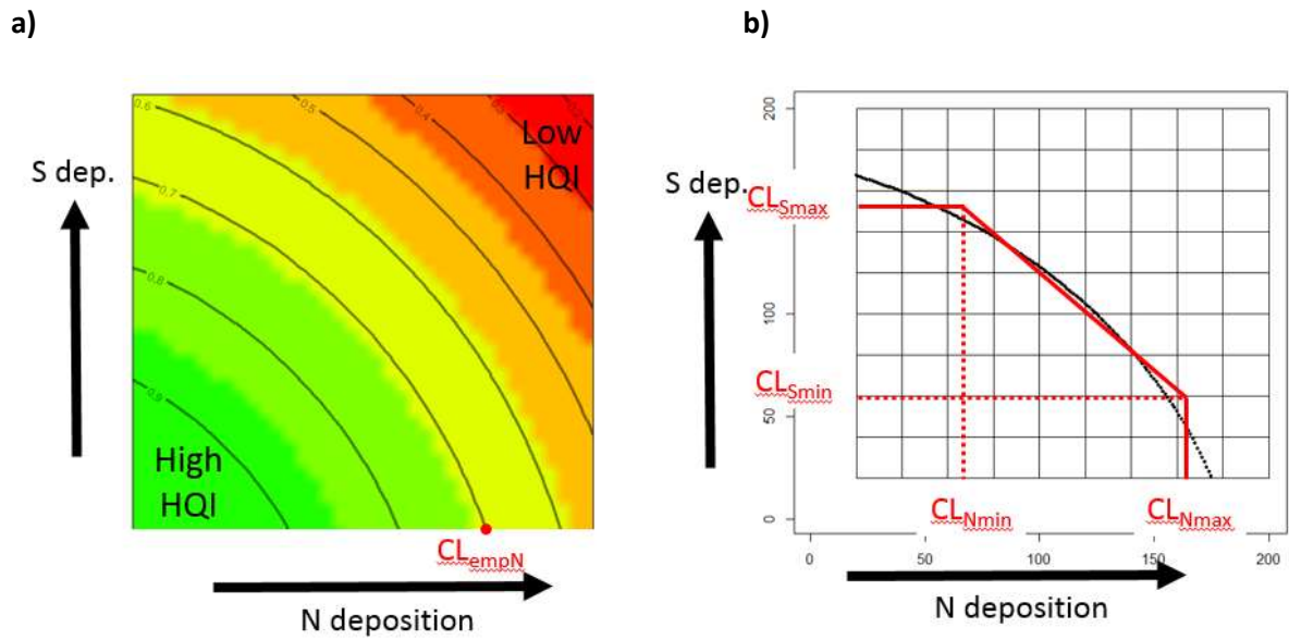
Figure 6.2: a) Response to combined loads of nitrogen and sulphur of a habitat quality index ( HQI ), as shown by colours and contours, at a hypothetical site; b) contour (black line) where HQI reaches a critical value, corresponding to a 'biodiversity-based' Critical Load function, and simplified version of this function by two points (red line).
