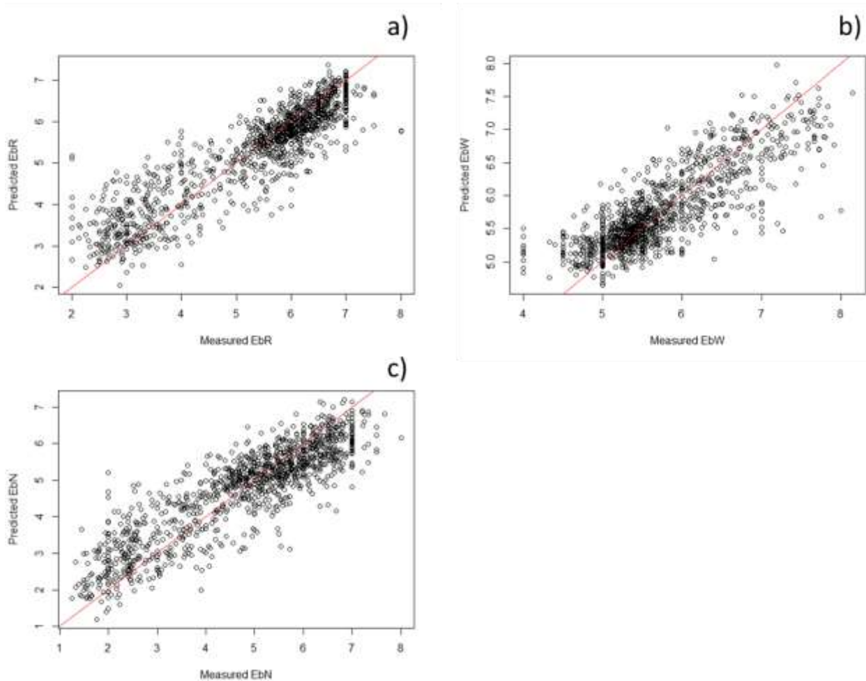
Figure 6.9: Model fits from multiple predictor equations for a) Ellenberg R, b) Ellenberg F, c) Ellenberg N
