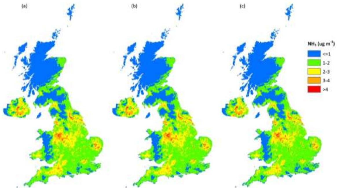
Figure 2.8. FRAME mean ammonia concentrations for (a) 2009-2011; (b) 2010-2012; (c) 2011-2013.
