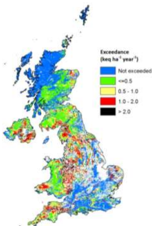
Figure 2: Average Accumulated Exceedance of acidity critical loads for all habitats combined by FRAME 2020 shipping scenario 1
