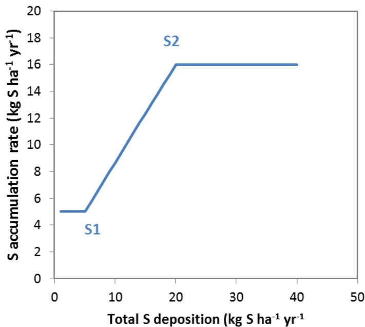
Figure 9.1: Response function for the relationship between peat S accumulation rate and total (marine plus non-marine) S deposition, based on peat core data (Section 9.2). Point S1 represents the S deposition at which the peat S accumulation begins to rise above background rates, and point S2 represents the S deposition at which the maximum rate of peat S accumulation occurs.
