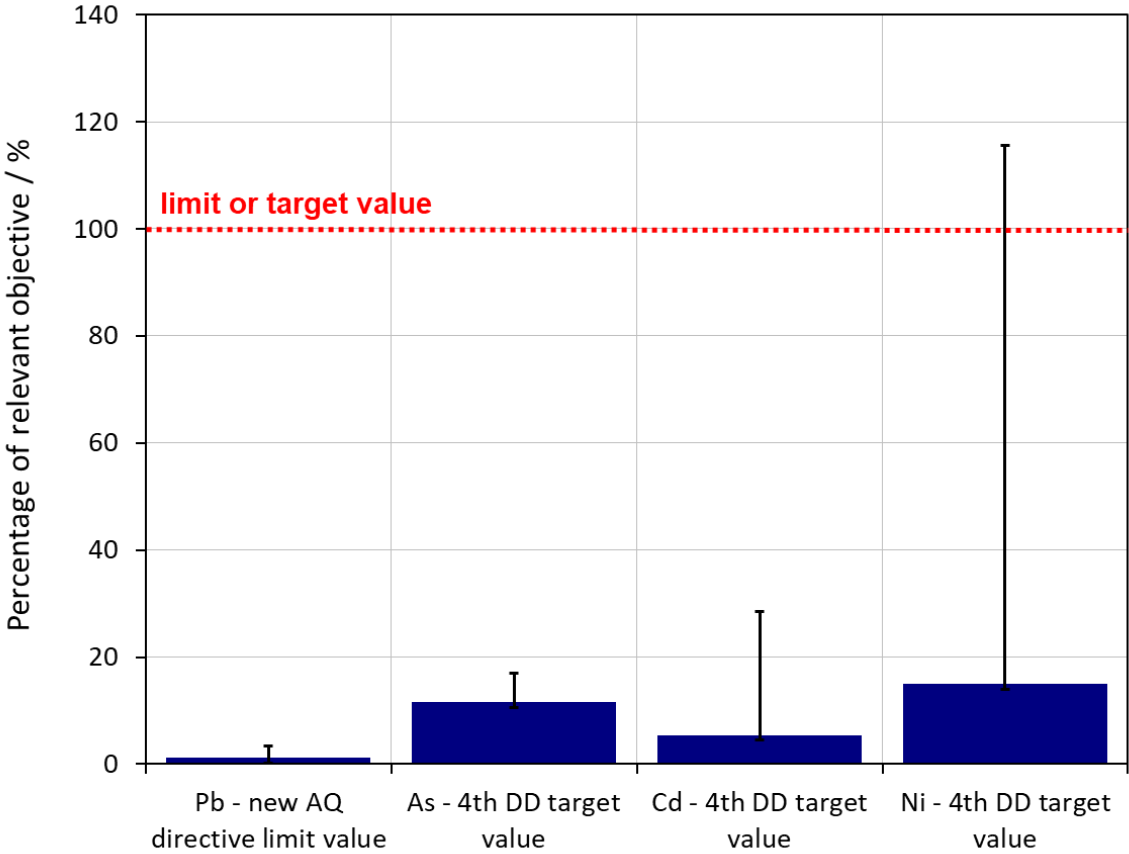
Figure 3 A summary of the annual mean measured concentrations of the heavy metals relevant to the Ambient Air Quality Directive and Fourth Daughter Directive on the UK Heavy Metals Monitoring Network in 2020 as a percentage of the relevant air quality objectives. The bars indicate the annual mean of all sites; the lines indicate the annual mean at the site with the highest concentrations.
