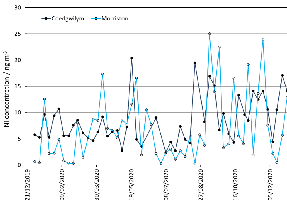
Figure 5 Measured Ni concentrations at Site 100: Swansea Coedgwilym and Site 101: Swansea Morryston, in 2020 (both sampled weekly).
