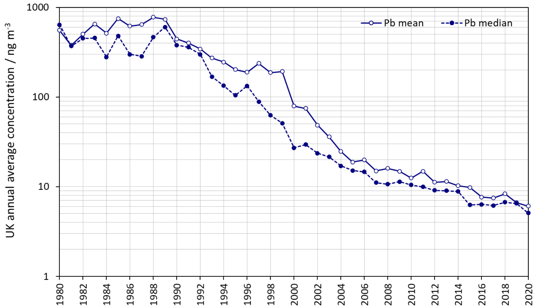
Figure 9 The mean and median of site annual average concentrations of Pb measured on the UK Heavy Metals Monitoring Network over the last 40 years. The EC limit value for lead is 500 ng m -3 and the UK Air Quality Objective for lead is 250 ng m -3 . Note the logarithmic scale on the y-axis.
